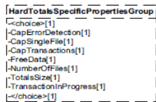
Figure 72: Hard Totals Properties Domain View
