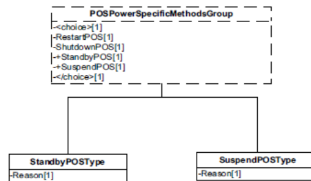
Figure 121: POS Power Methods Domain View
