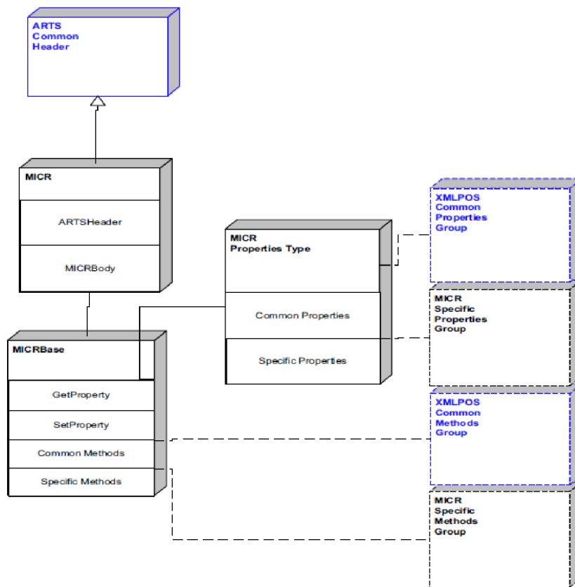
Figure 95: MICR Domain View
