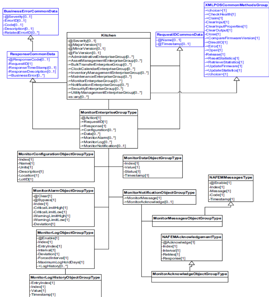
Figure 161: Monitor Enterprise Group Domain View
