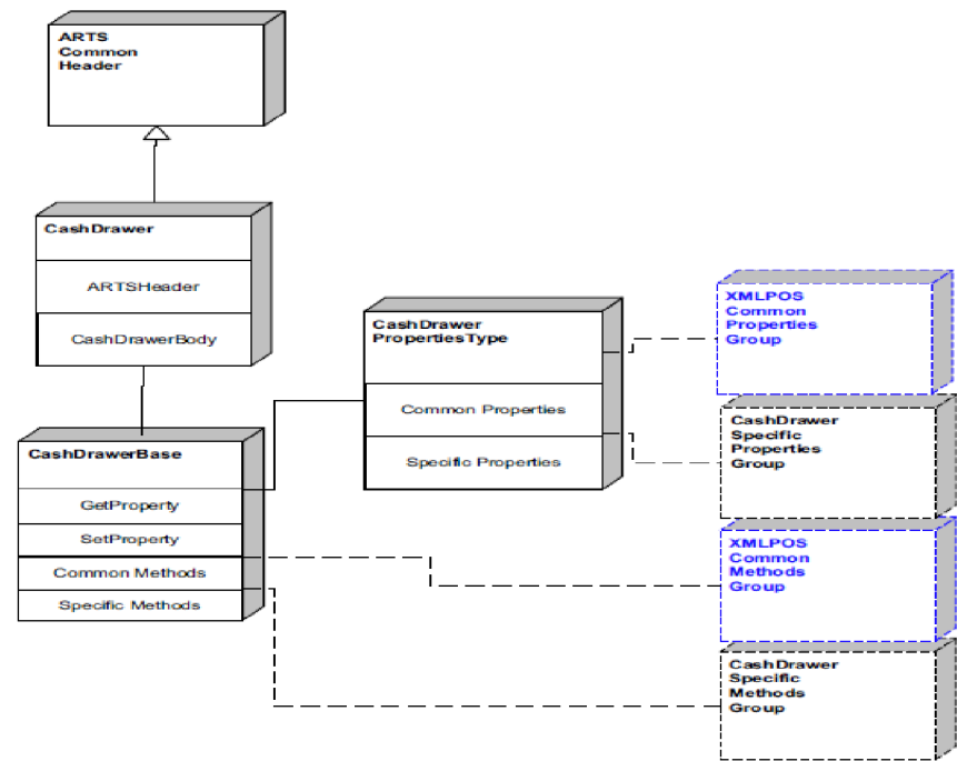
Figure 35: Cash Drawer Domain View
