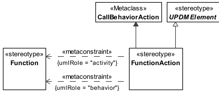
Figure 8.115 - FunctionAction
