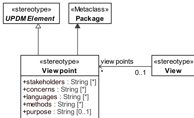
Figure 8.35 - Viewpoint
