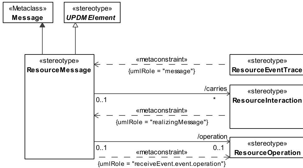
Figure 8.118 - ResourceMessage
