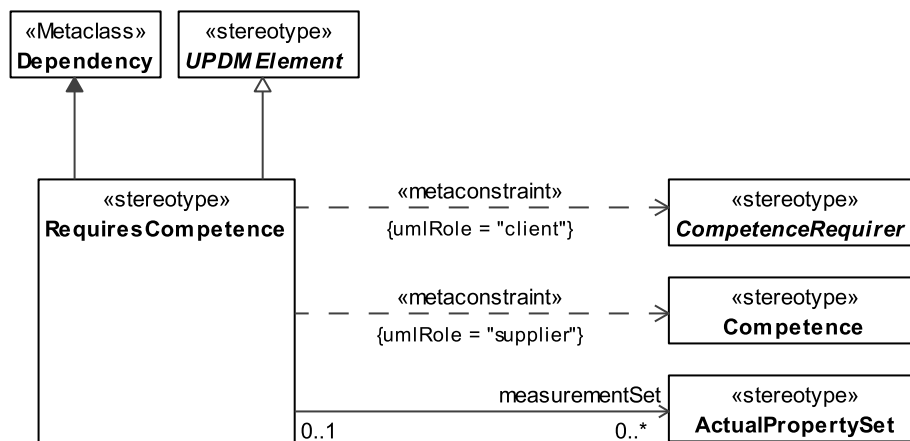
Figure 8.81 - RequiresCompetence
