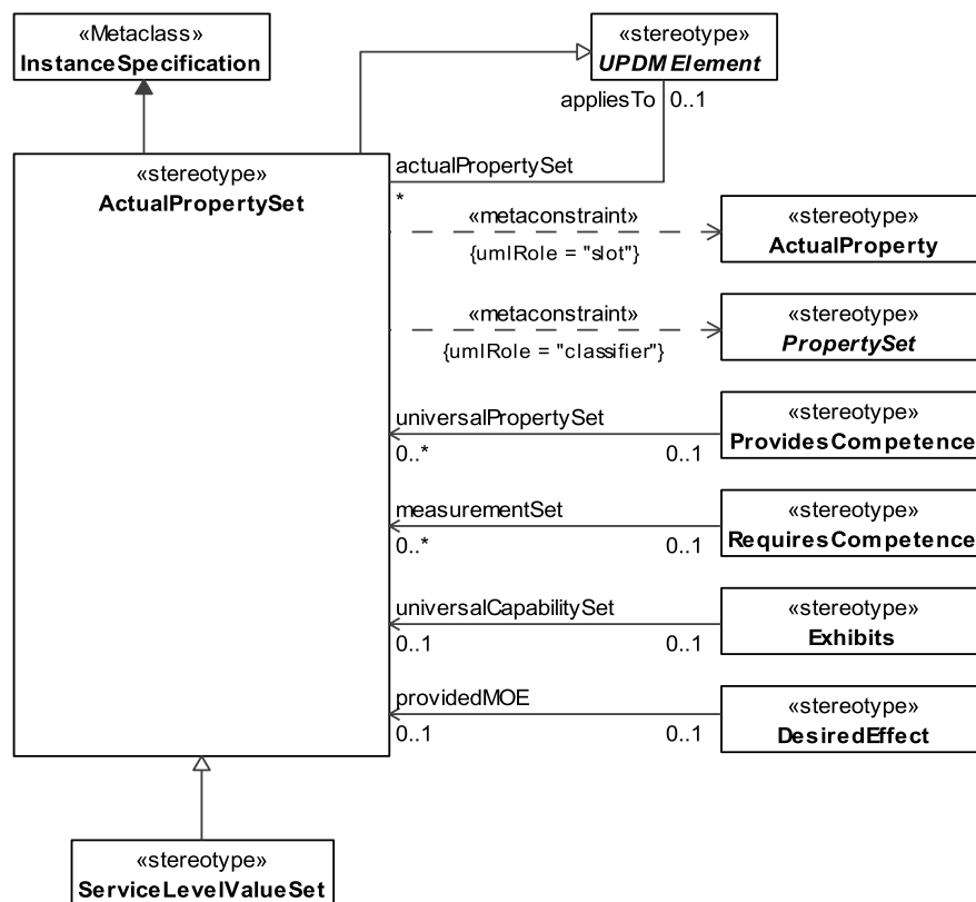
Figure 8.21 - ActualPropertySet
