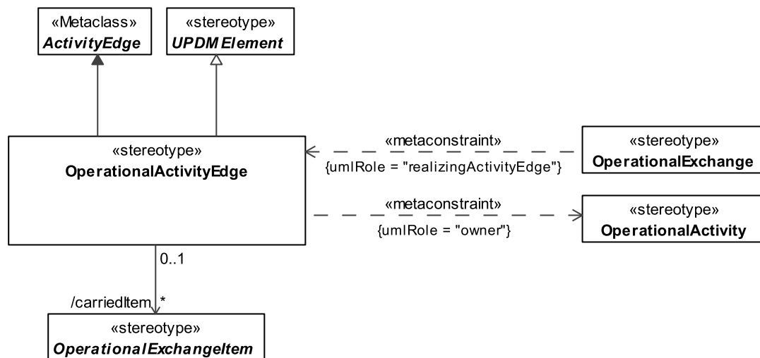
Figure 8.40 - OperationalActivityEdge
