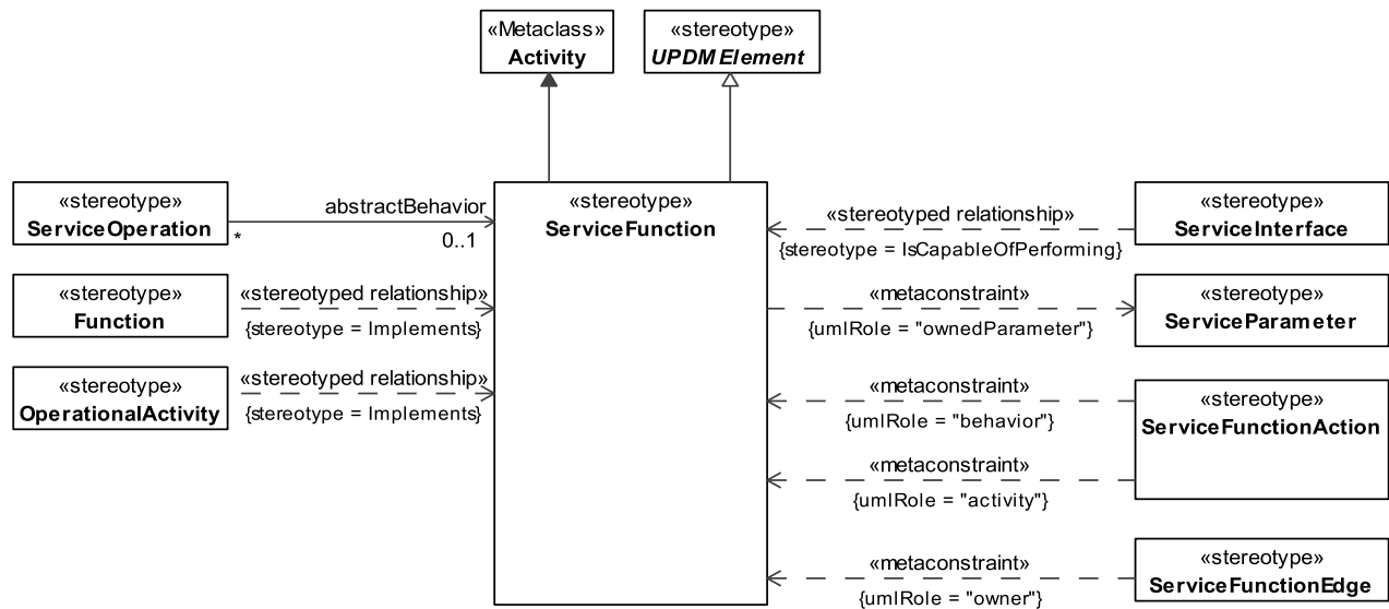
Figure 8.84 - ServiceFunction
