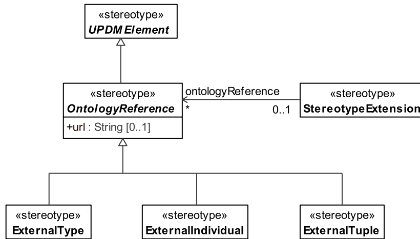
Figure 8.199 - OntologyReference
