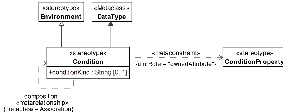
Figure 8.159 Condition
