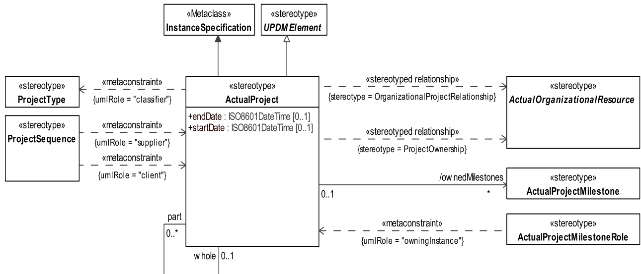
Figure 8.2 - ActualProject
