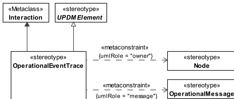
Figure 8.41 - OperationalEventTrace
