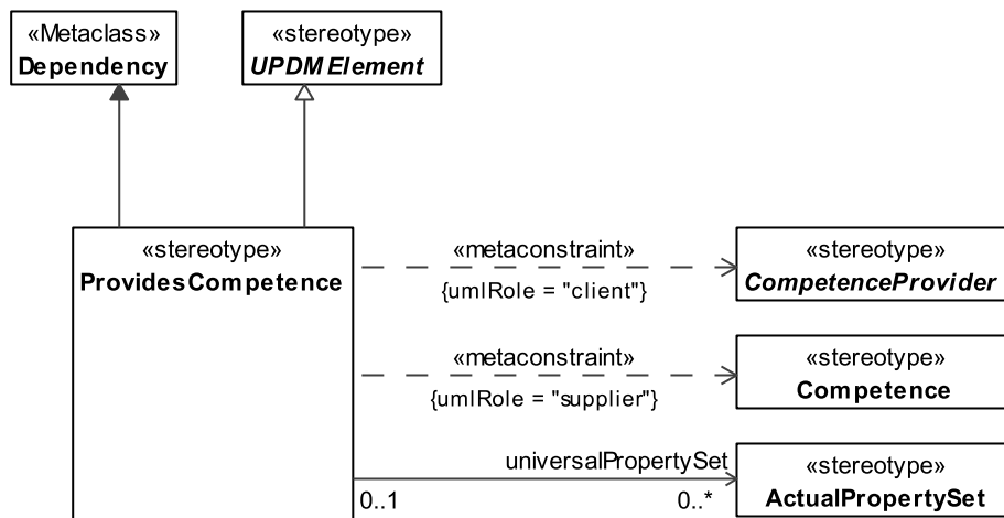
Figure 8.80 - ProvidesCompetence
