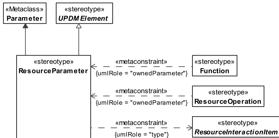
Figure 8.120 - ResourceParameter
