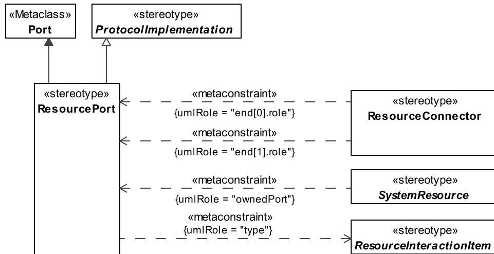
Figure 8.136 - ResourcePort
