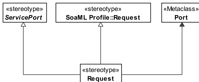
Figure 8.94 - Request
