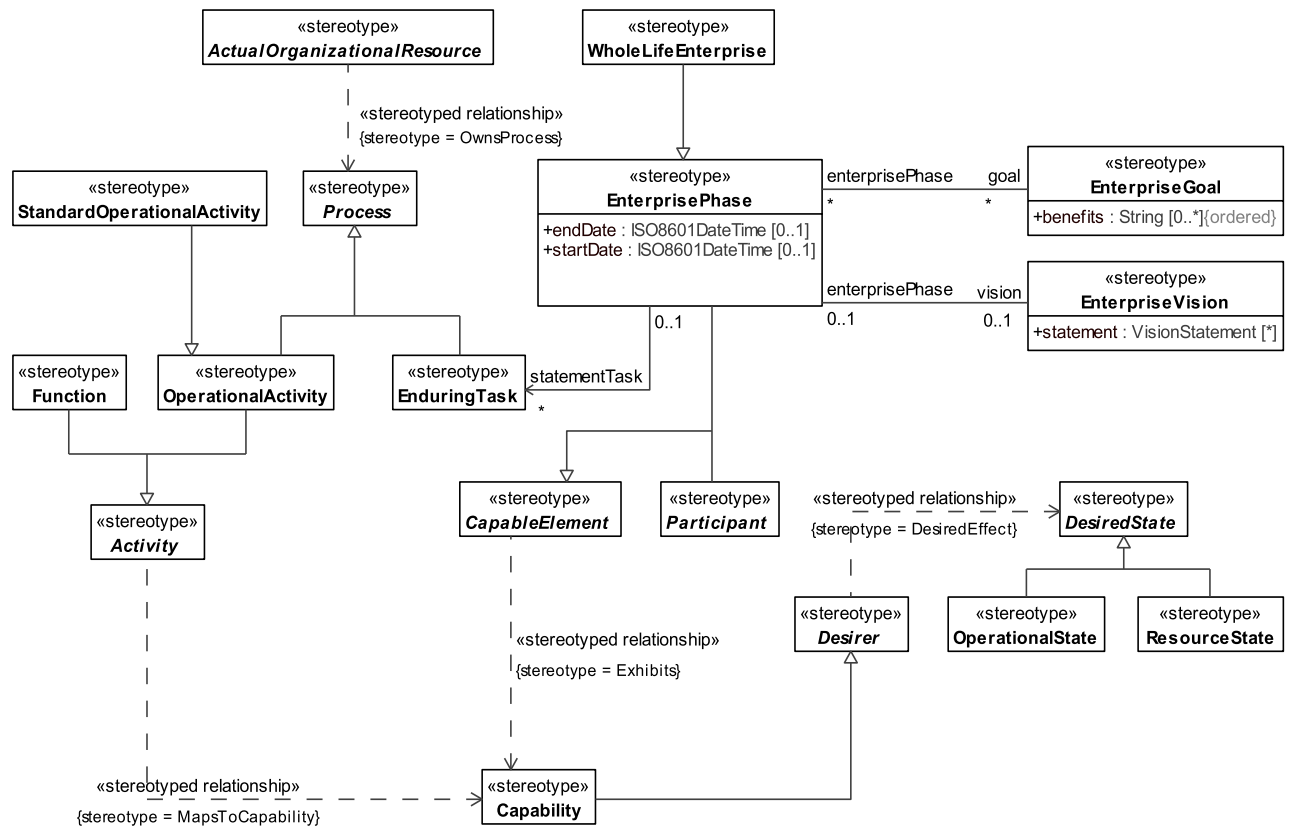
Figure B.27 - StV-1/CV-1
