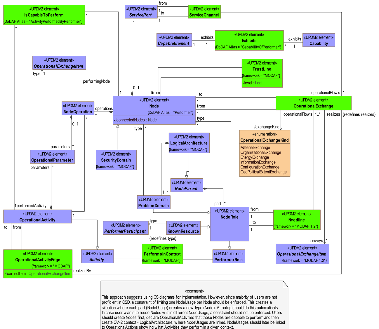
Figure A.9 - OV-2 - DMM
