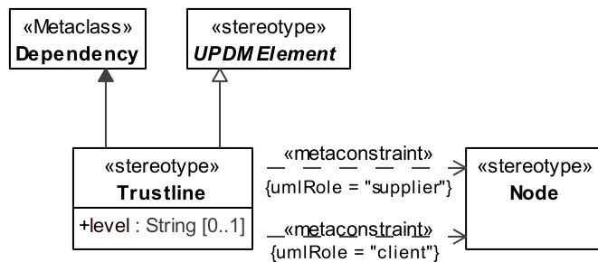
Figure 8.209 - Trustline
