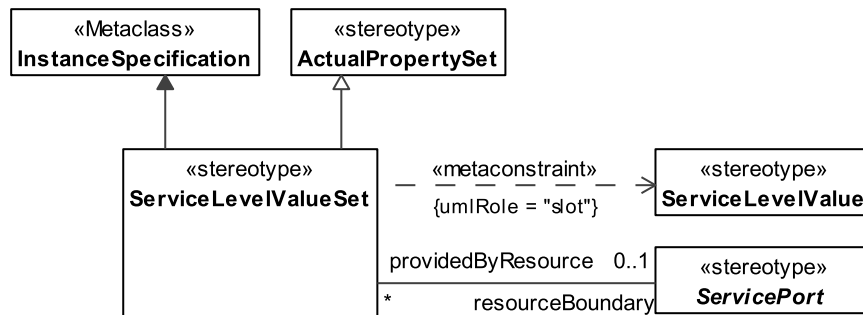
Figure 8.99 - ServiceLevelValueSet
