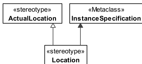
Figure 8.163 - Location
