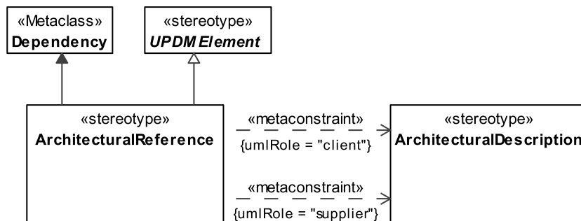
Figure 8.31 - ArchitecturalReference
