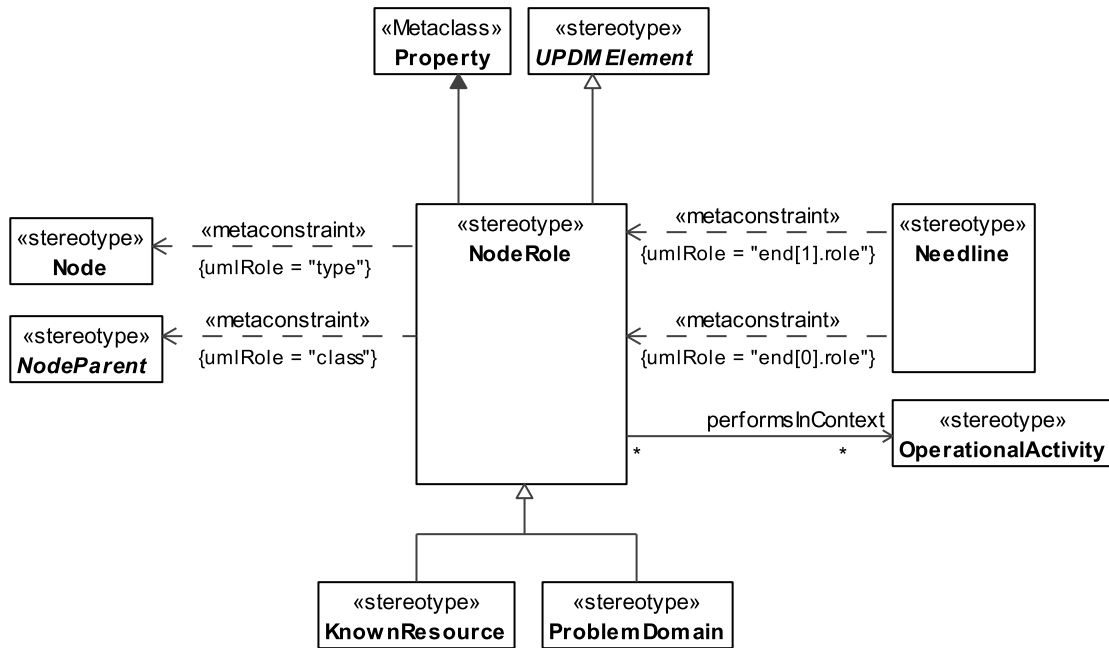
Figure 8.63 - NodeRole
