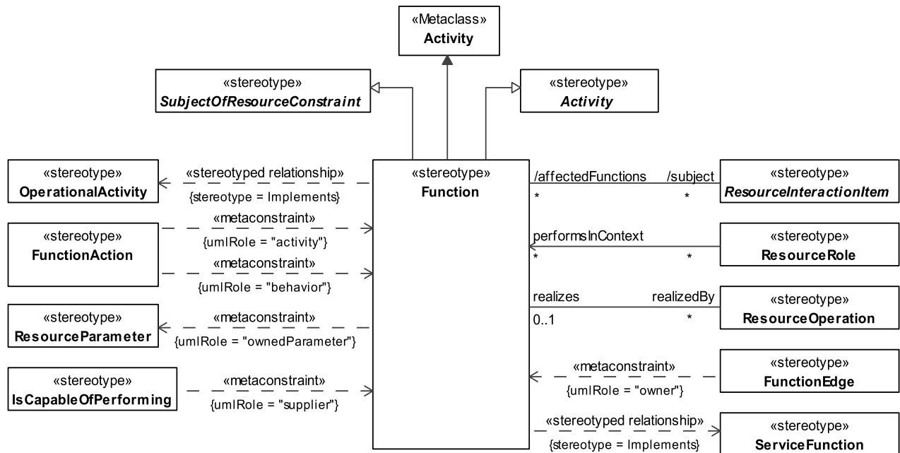
Figure 8.114 - Function
