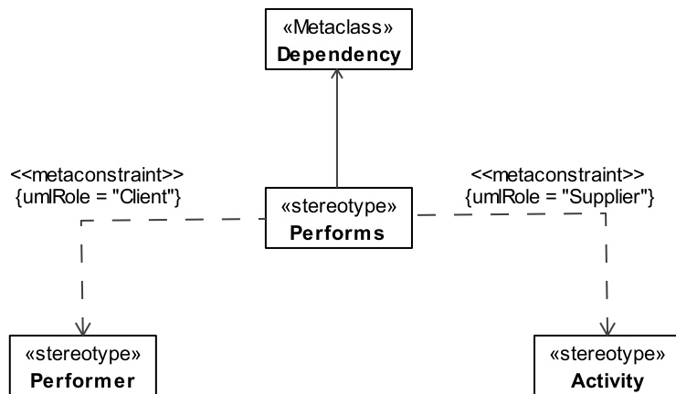
Figure 7.2 - Performs Hierarchy
