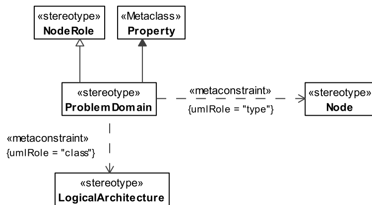
Figure 8.208 - ProblemDomain
