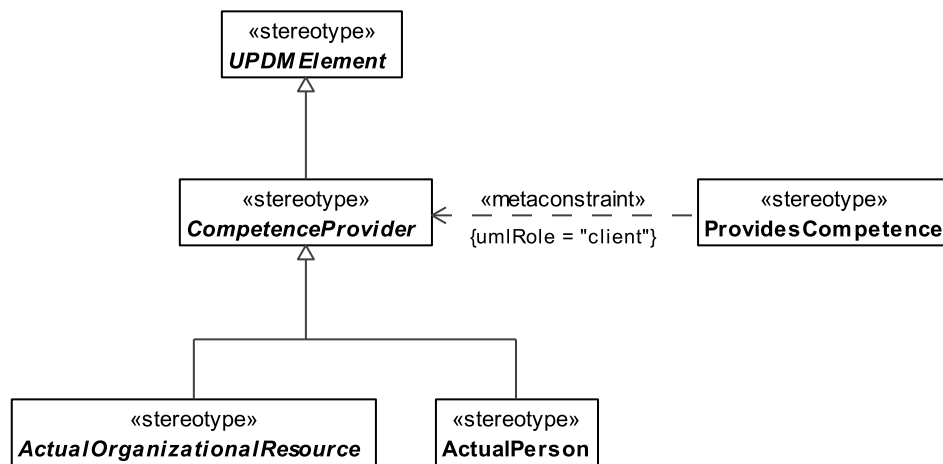
Figure 8.73 - CompetenceProvider
