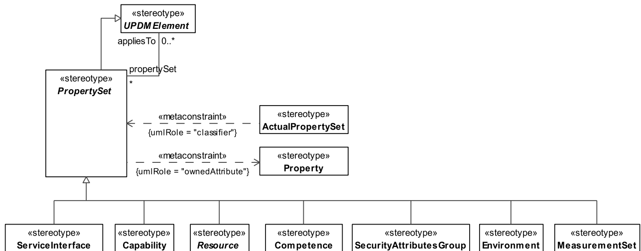
Figure 8.25 - PropertySet
