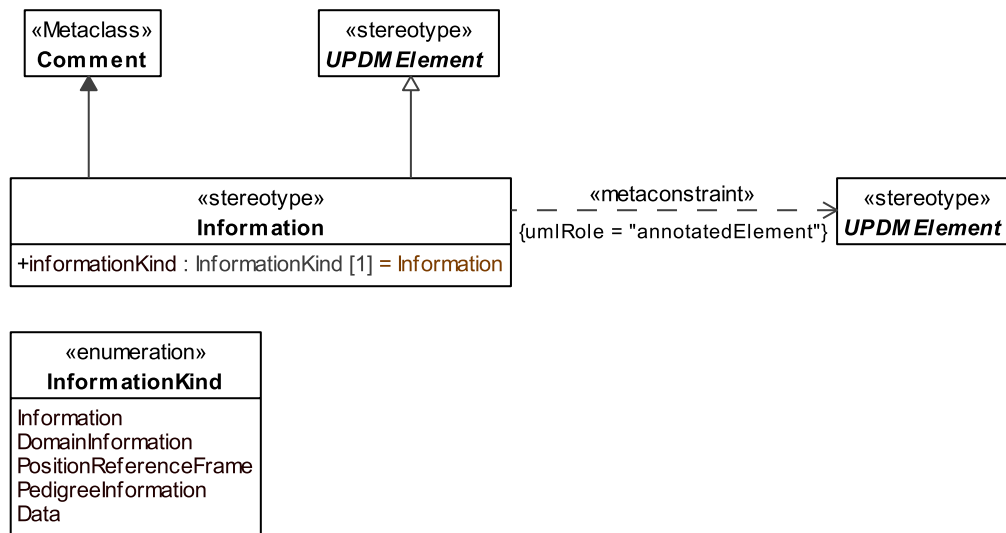
Figure 8.157 - Information
