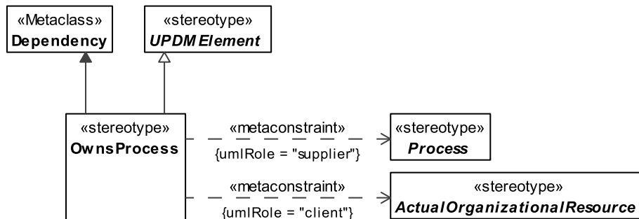
Figure 8.203 - OwnsProcess
