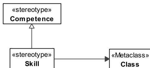
Figure 8.170 - Skill
