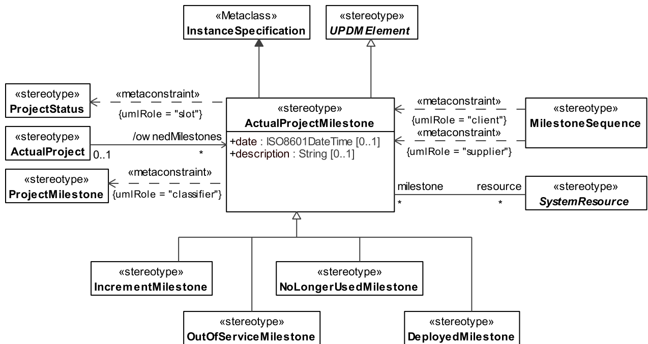
Figure 8.183 - ActualProjectMilestone
