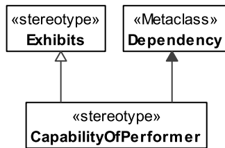
Figure 8.175 - CapabilityOfPerformer
