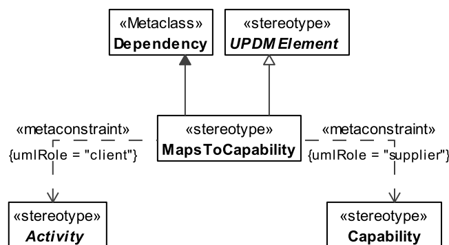
Figure 8.110 - MapsToCapability
