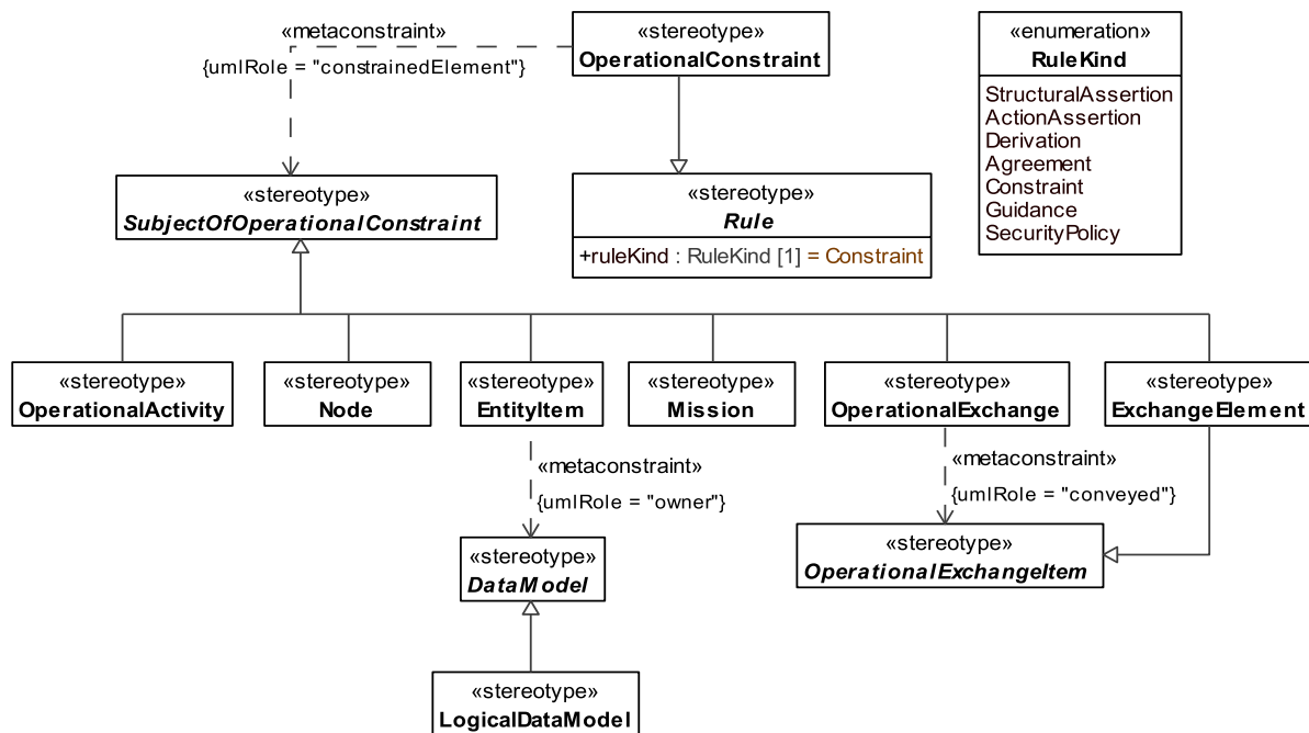
Figure B.15 - OV-6a
