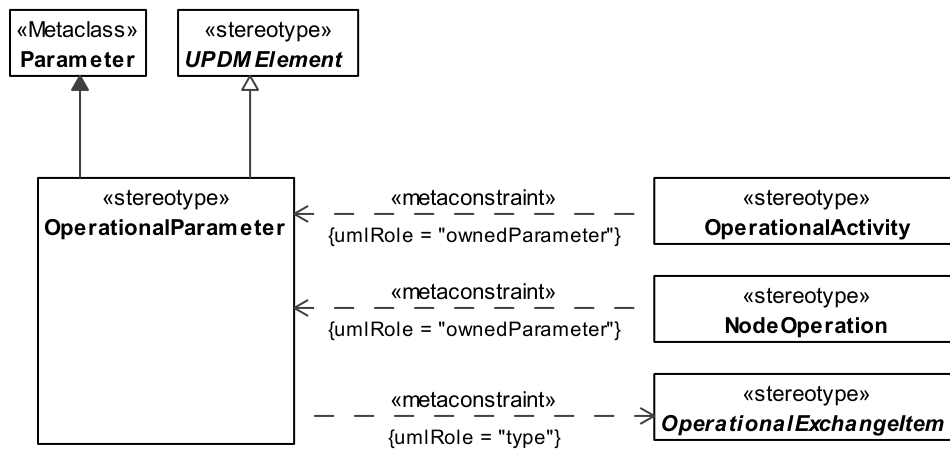
Figure 8.43 - OperationalParameter
