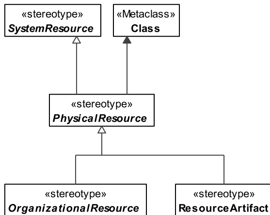
Figure 8.131 - PhysicalResource
