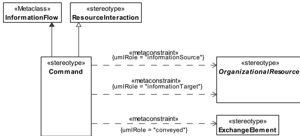
Figure 8.48 - Command
