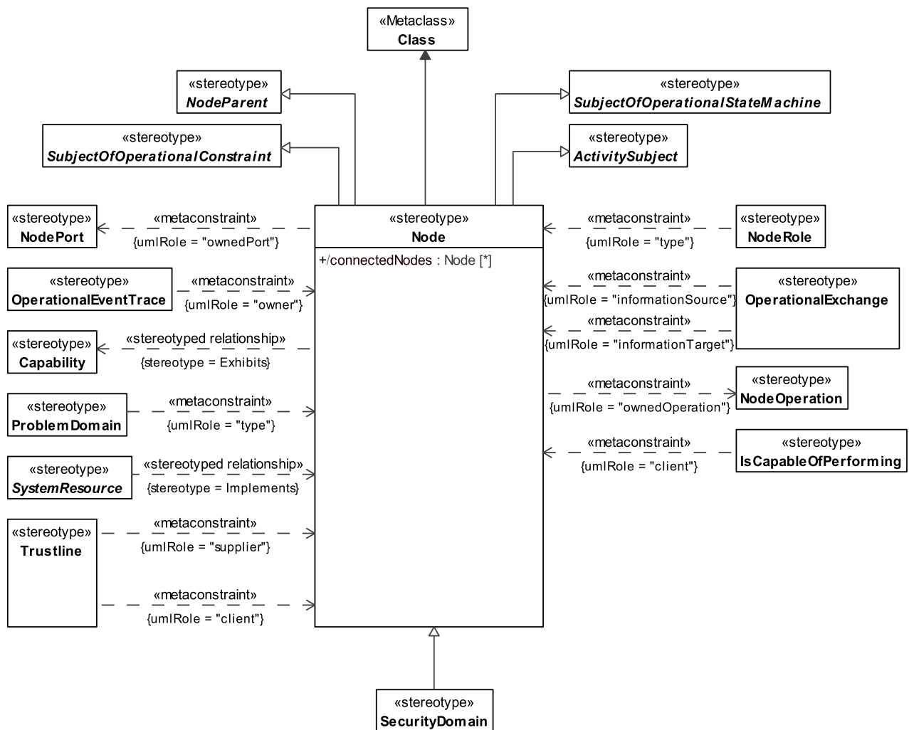
Figure 8.60 - Node
