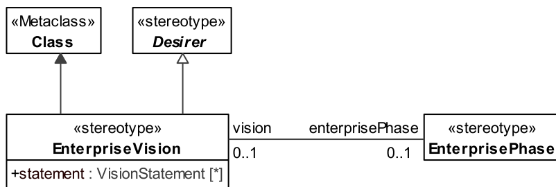
Figure 8.108 - EnterpriseVision
