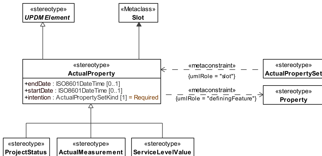
Figure 8.20 - ActualProperty
