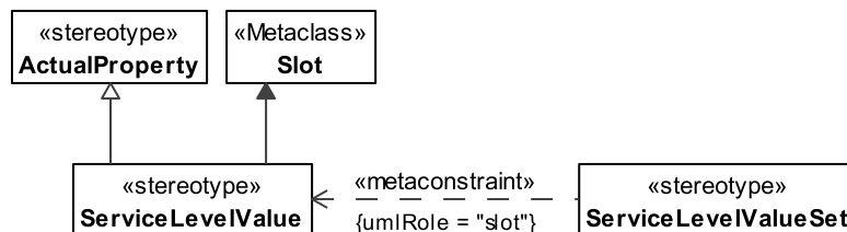
Figure 8.98 - ServiceLevelValue
