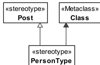
Figure 8.169 - PersonType
