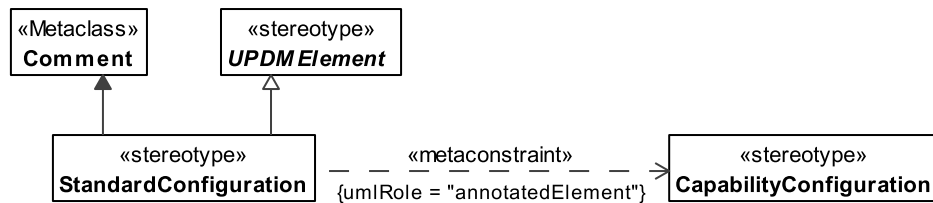
Figure 8.147 - StandardConfiguration
