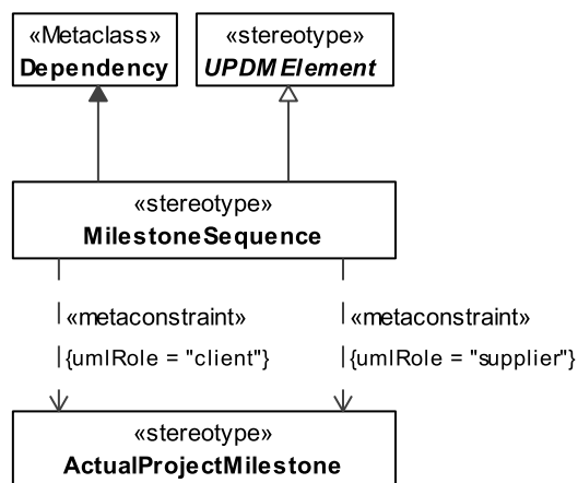
Figure 8.185 - MilestoneSequence
