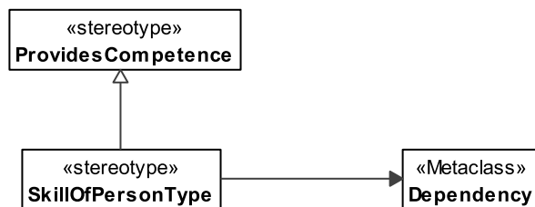
Figure 8.171 - SkillOfPersonType
