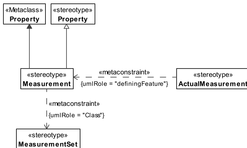
Figure 8.22 - Measurement
