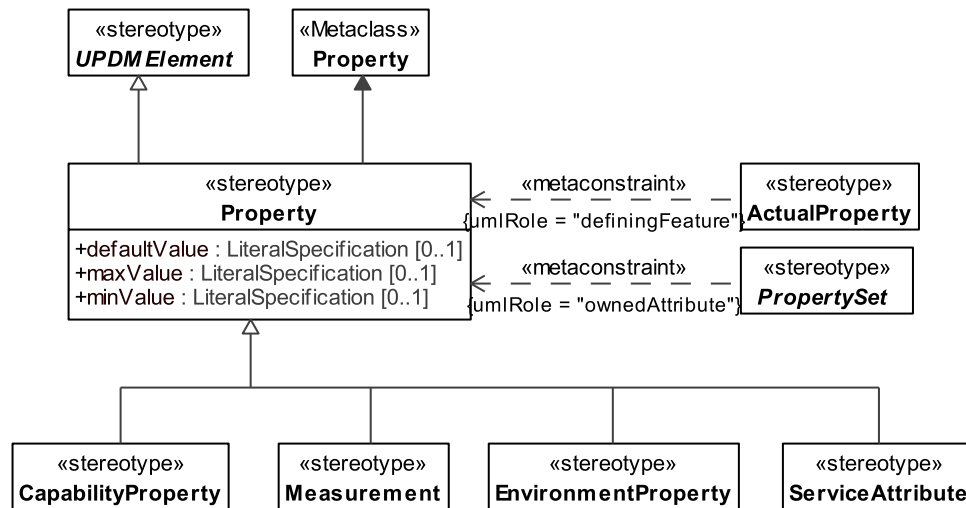
Figure 8.24 - Property
