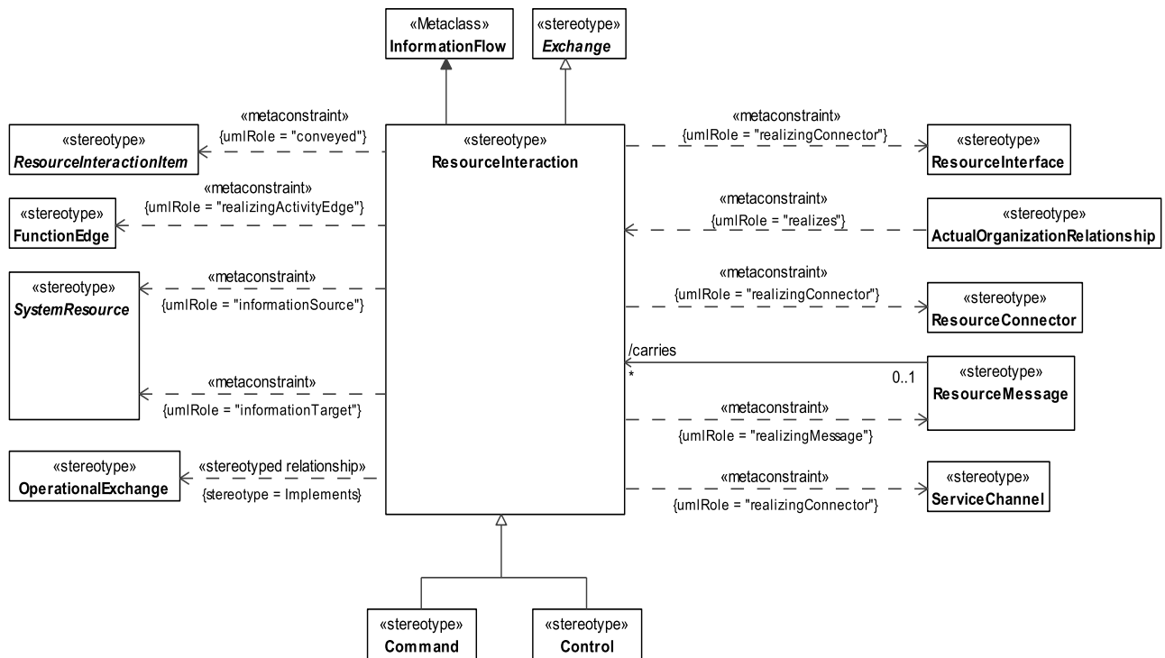
Figure 8.125 - ResourceInteraction
