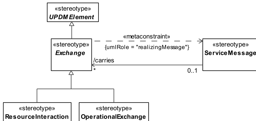
Figure 8.7 - Exchange
