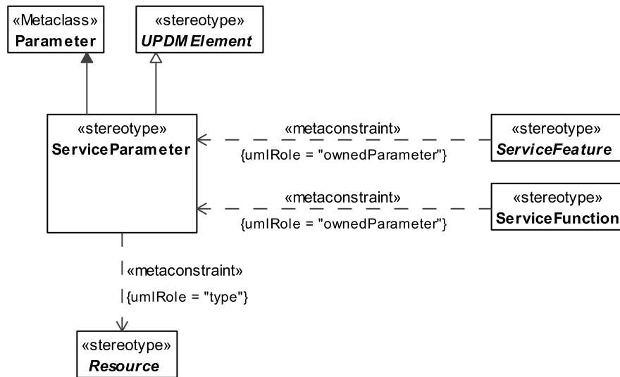
Figure 8.91 - ServiceParameter
