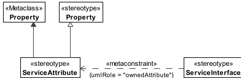
Figure 8.96 - ServiceAttribute
