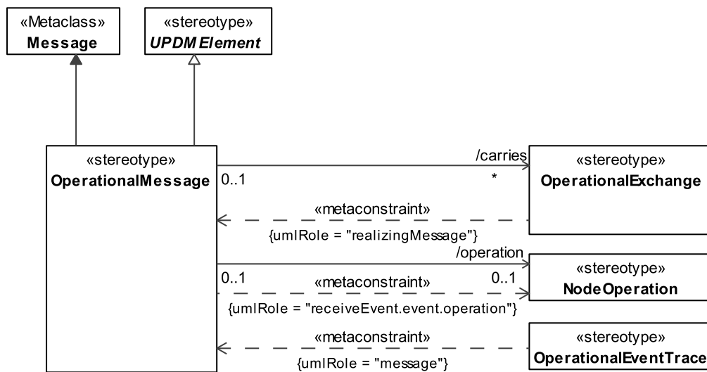
Figure 8.42 - OperationalMessage
