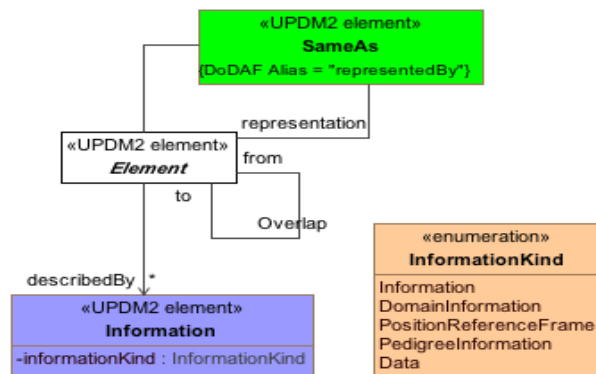
Figure A.52 - Information Pedigree - DM2
