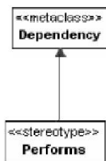
Figure 7.1 - Performs Stereotype
