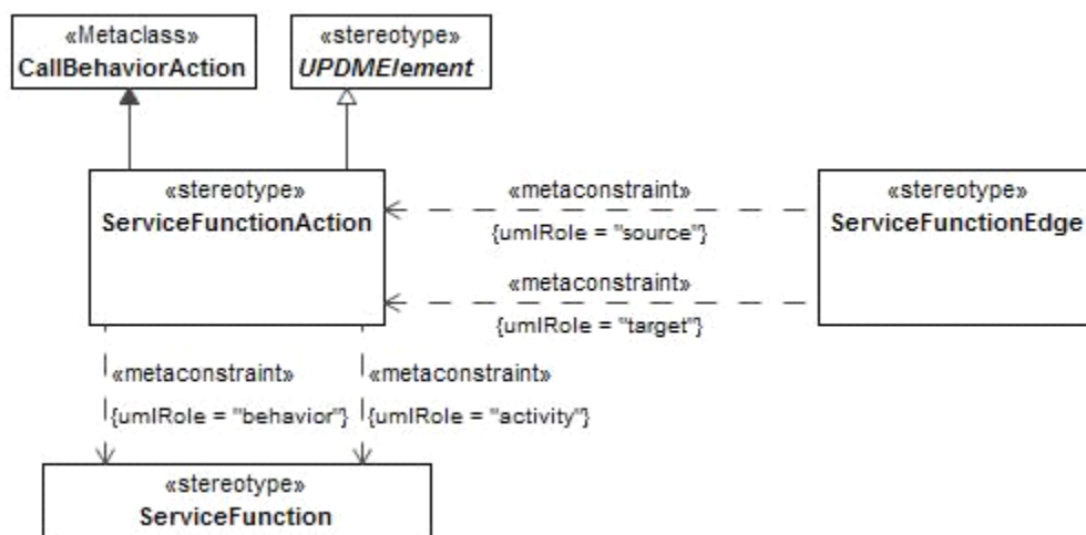
Figure 8.85 - ServiceFunctionAction
