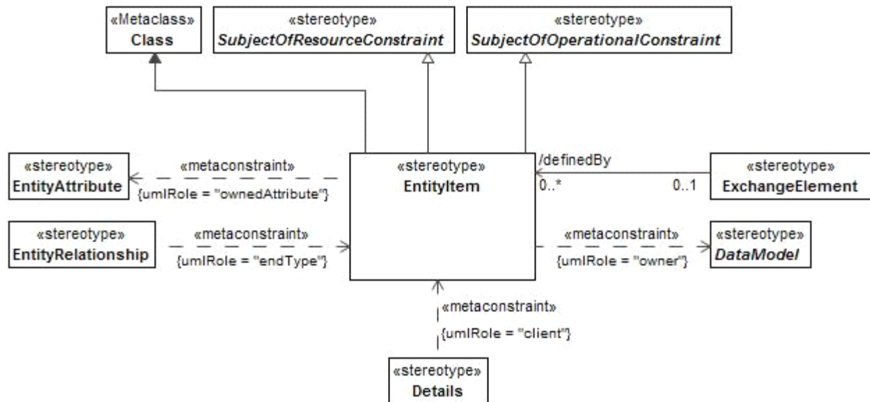
Figure 8.150 - EntityItem
