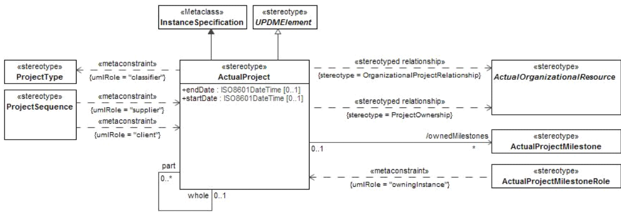
Figure 8.2 - ActualProject
