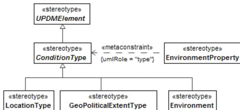
Figure 8.14 - ConditionType
