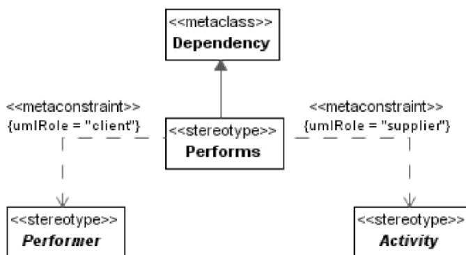
Figure 7.2 - Performs Hierarchy
