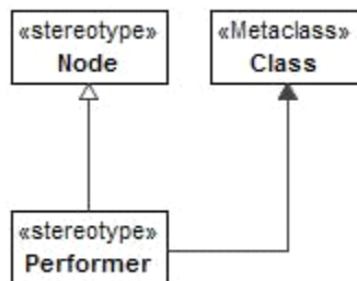
Figure 8.166 - Performer
