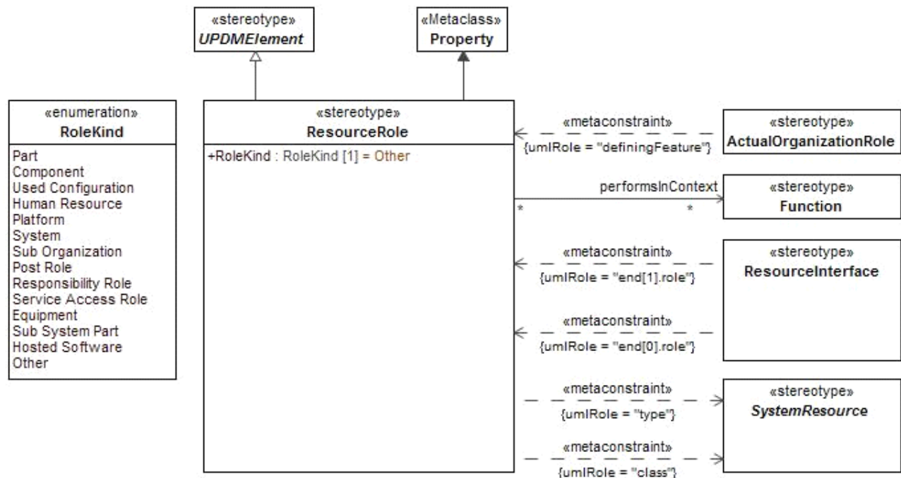
Figure 8.137 - ResourceRole
