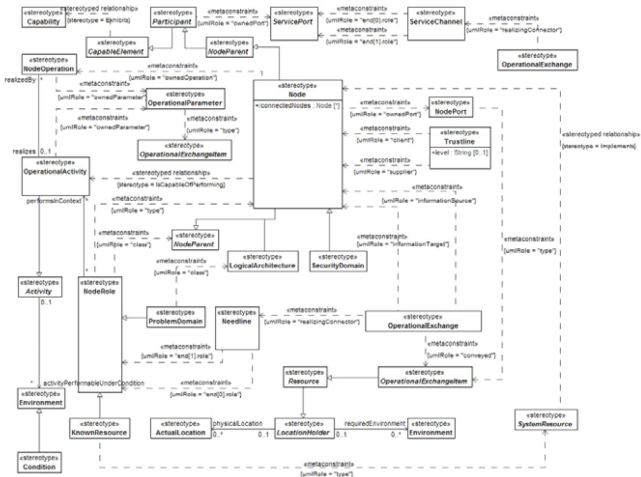
Figure B.10 - OV-2
