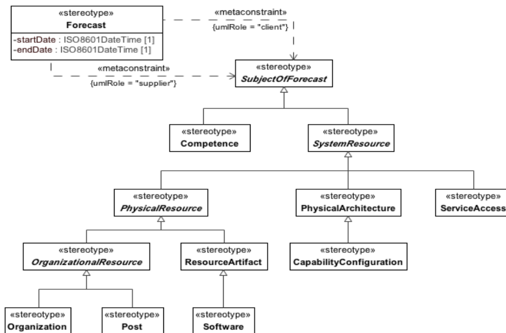
Figure B.46 - SV-9/SvcV-9
