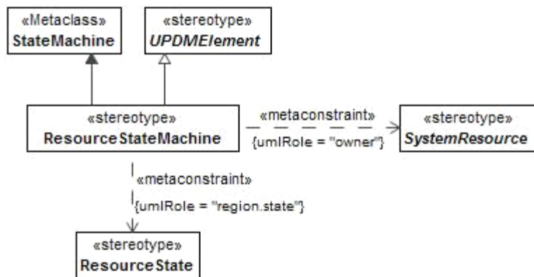
Figure 8.122 - ResourceStateMachine
