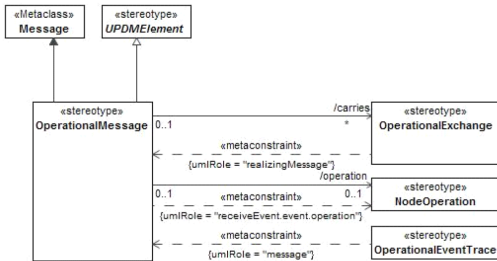
Figure 8.42 - OperationalMessage
