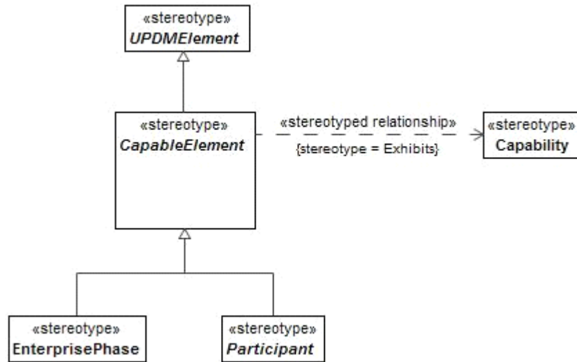
Figure 8.10 - CapableElement
