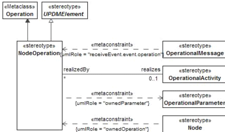
Figure 8.37 - NodeOperation
