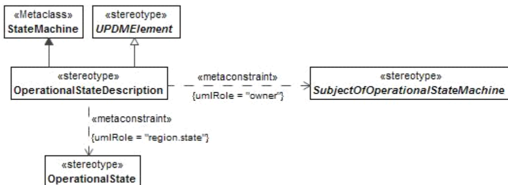
Figure 8.45 - OperationalStateDescription
