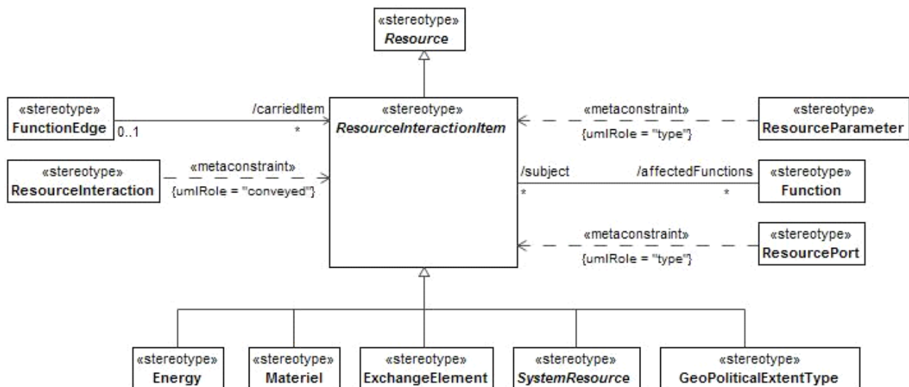
Figure 8.126 - ResourceInteractionItem
