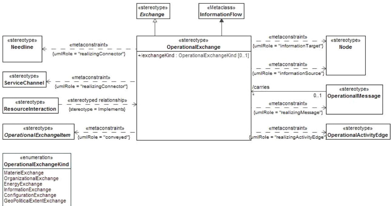
Figure 8.49 - OperationalExchange
