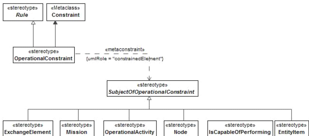
Figure 8.64 - OperationalConstraint
