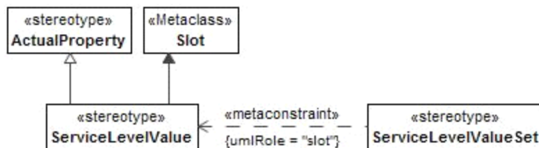
Figure 8.98 - ServiceLevelValue
