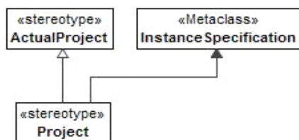
Figure 8.153 - Project
