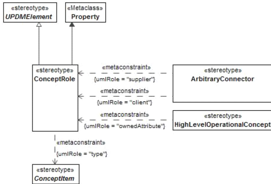
Figure 8.54 - ConceptRole
