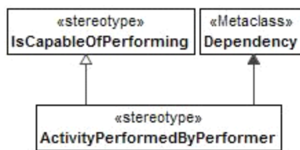
Figure 8.158 - ActivityPerformedByPerformer
