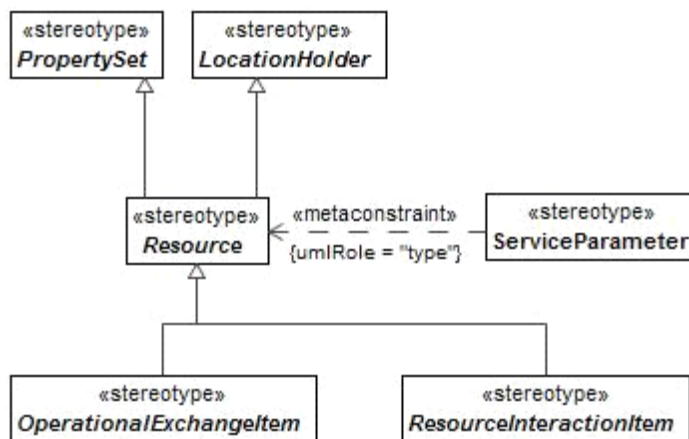
Figure 8.28 - Resource
