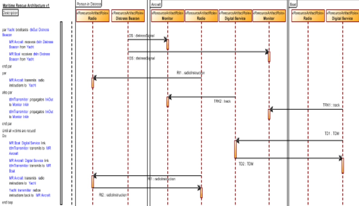
Figure D.38 - SV-10c
