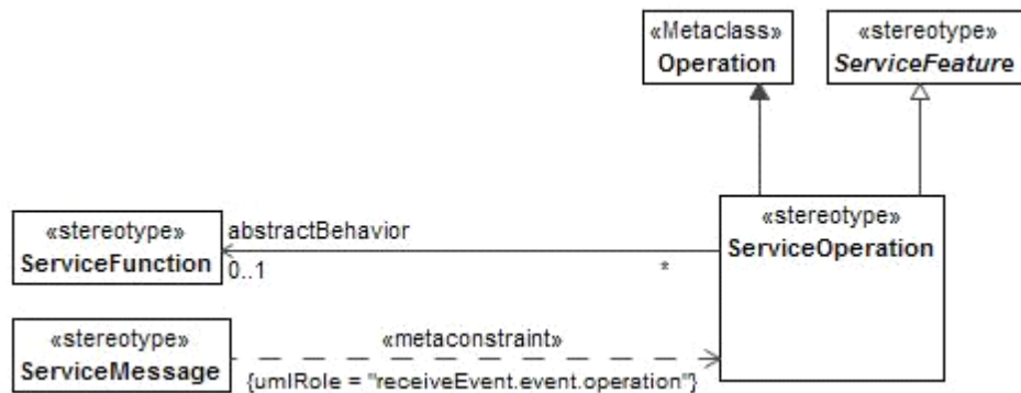
Figure 8.90 - ServiceOperation
