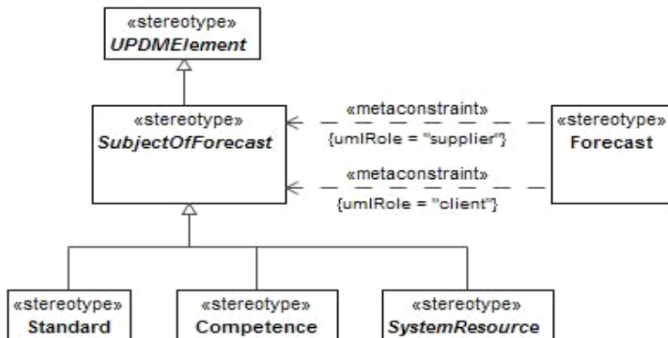
Figure 8.139 - SubjectOfForecast
