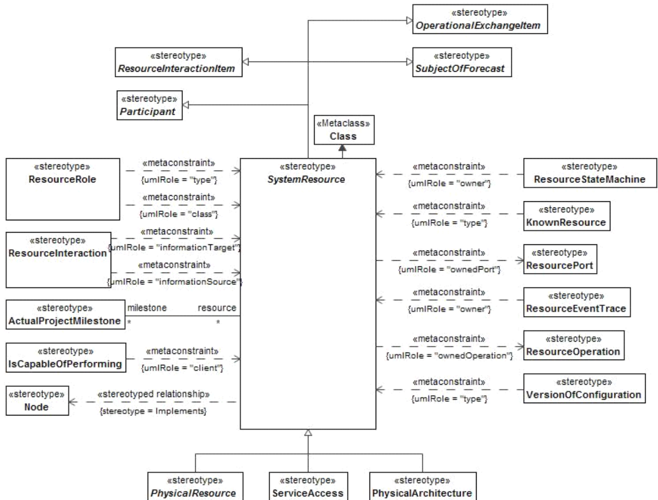
Figure 8.141 - SystemResource
