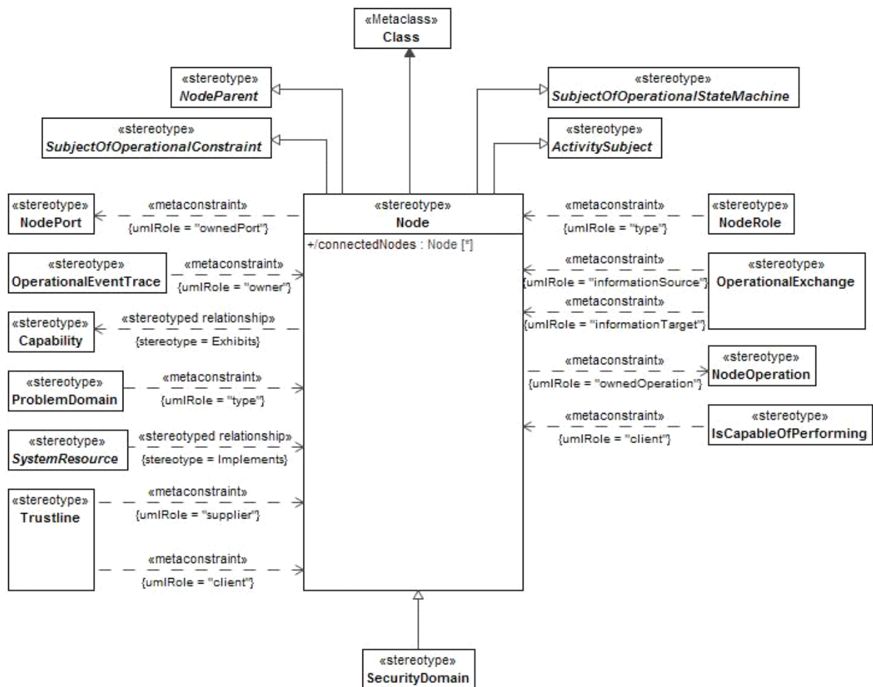
Figure 8.60 - Node
