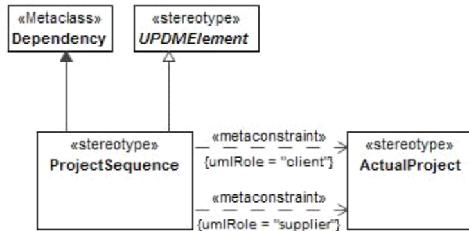
Figure 8.189 - ProjectSequence
