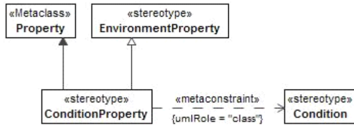
Figure 8.160 - ConditionProperty
