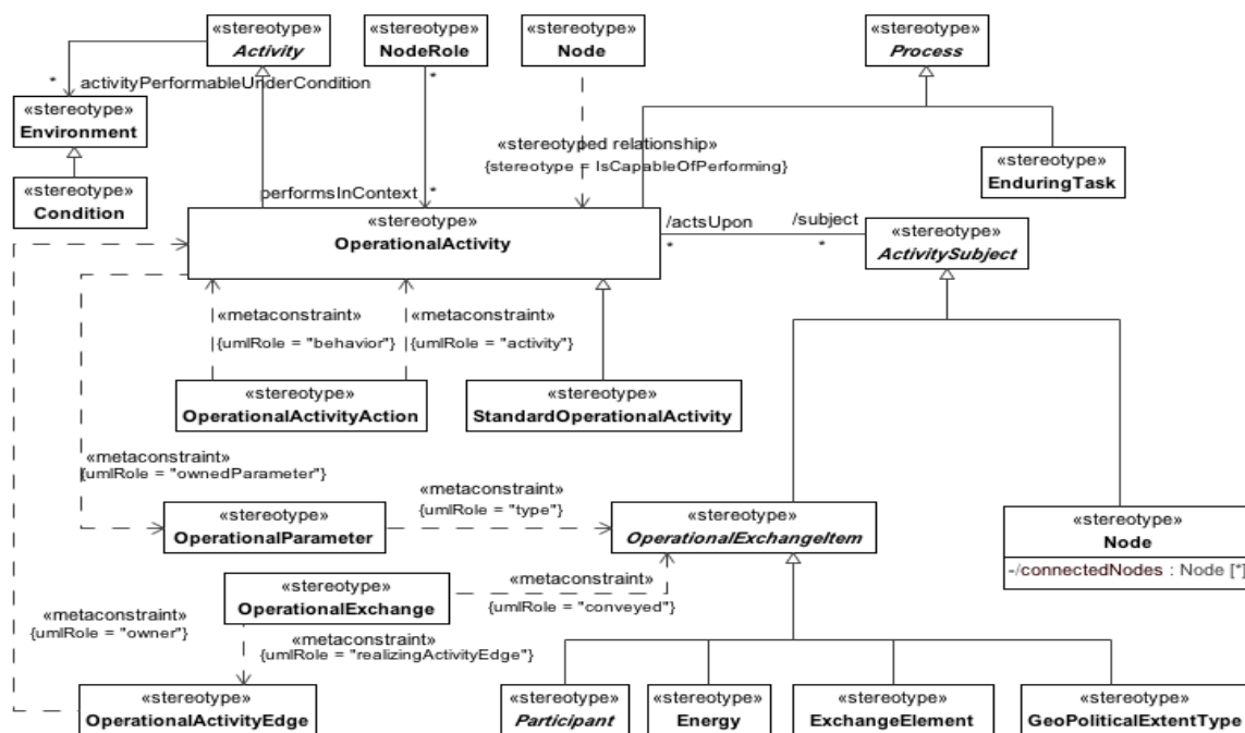
Figure B.14 - OV-5
