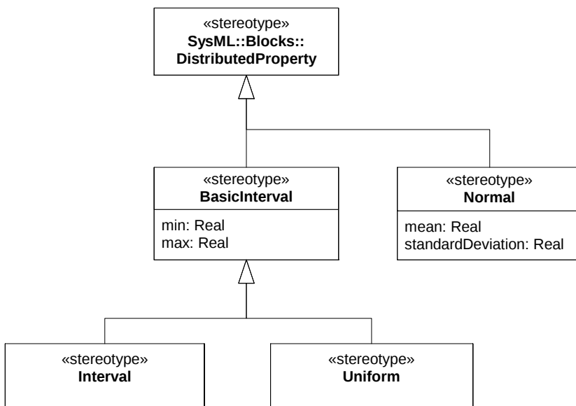
Figure E.21 - Basic distribution stereotypes
