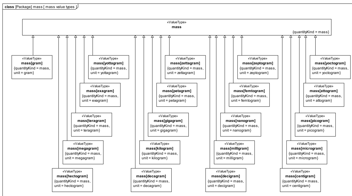
Figure E.20 - Example of value type definitions for a quantity and applicable units and prefixed units
