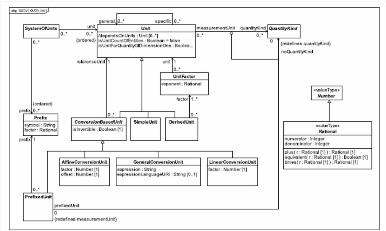
Figure E.6 - QUDV Units diagram
