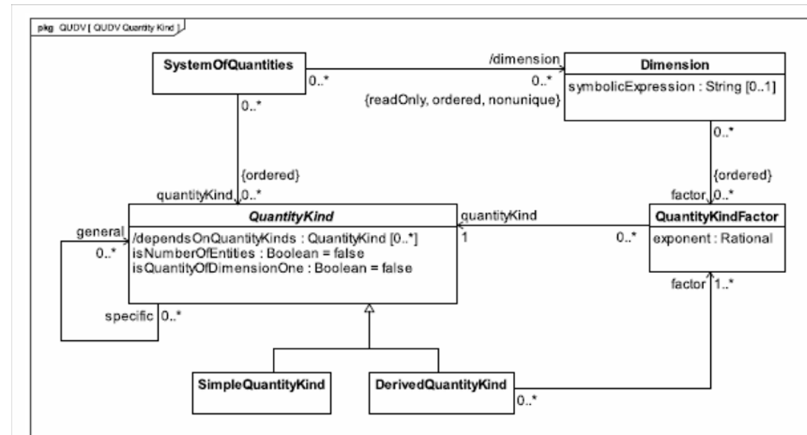
Figure E.7 - QUDV Quantity Kinds diagram
