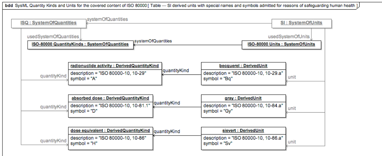
Figure E.18 - Table 3 (from the SI brochure) SI derived units with special names and symbols
