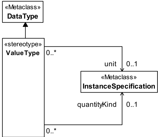
Figure 8.4 - Abstract syntax extensions for SysML value types
