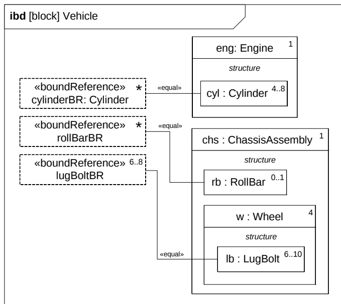
Figure 8.16 - Vehicle internal structure
