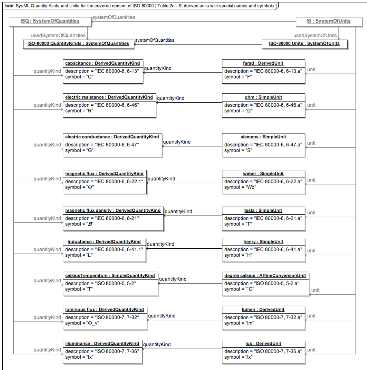
Figure E.17 - Table 2 (from ISO 80000-1) ISQ derived quantities and SI derived units with special names (3)
