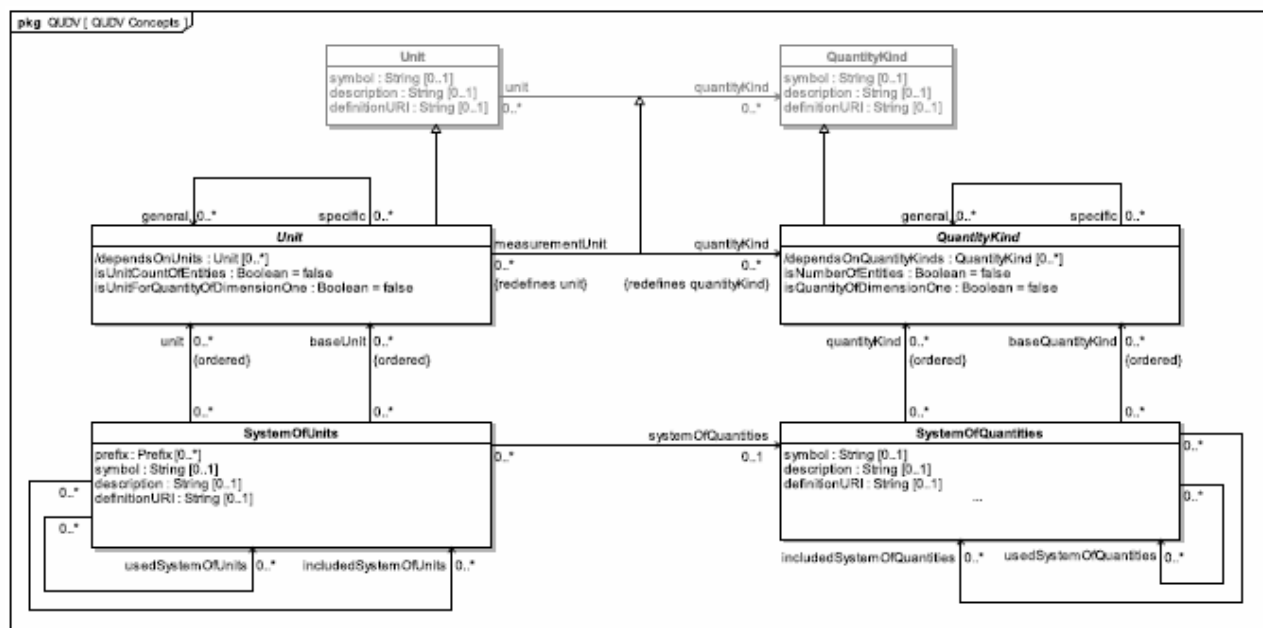
Figure E.5 - QUDV Concepts diagram
