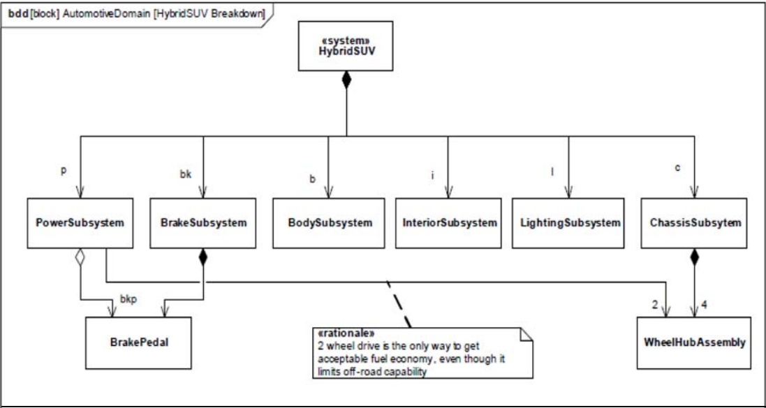
Figure D.16 - Defining Structure of the Hybrid SUV System (Block Definition Diagram)
