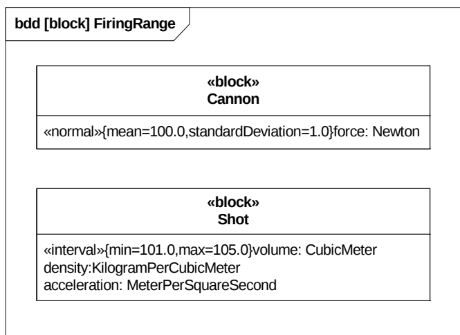
Figure E.22 - Distribution Example
