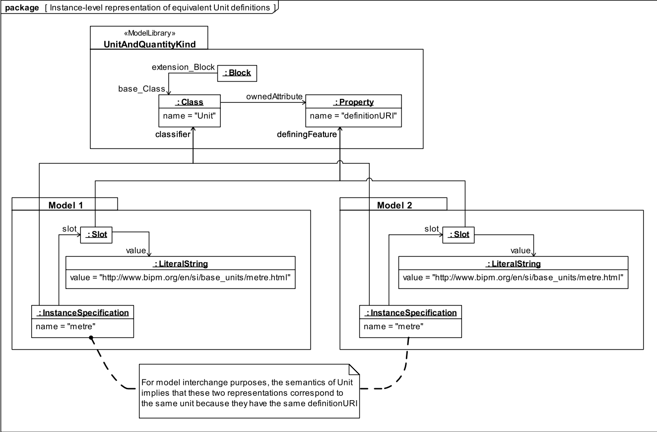
Figure 8.21 - Instance-level representation of equivalent Unit definitions
