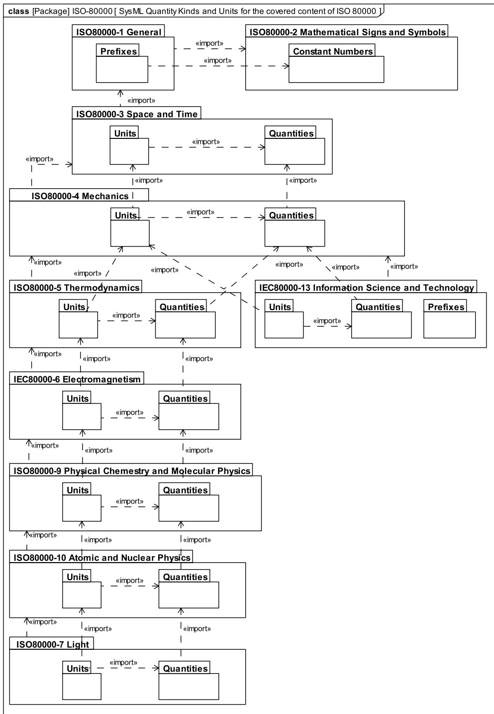
Figure E.12 - Organization of the definitions of units and quantities from the normative parts of ISO 80000 covered in SysML 1.4, which includes all the normative content of parts 3,4,5,6; the subset of parts 7,9,10 corresponding to the content from SysML 1.3 and the subset of part 13 pertaining to commonly used units of information. Parts 8,11 and 12 are not covered because none of their units and quantities were referenced in previous versions of SysML nor in the summary tables in ISO 80000-1
