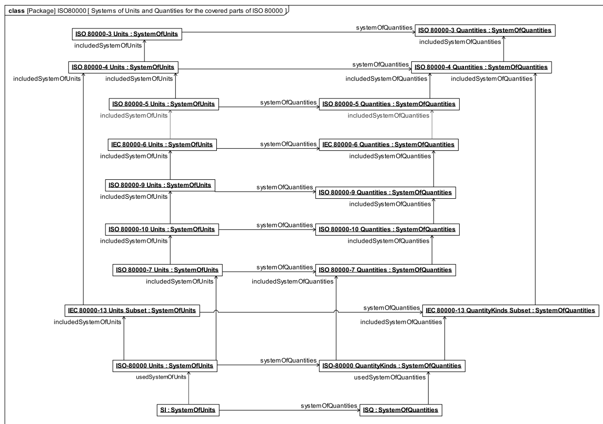
Figure E.13 - Content relationships for the systems of units and quantities in from the different parts of ISO 80000 in relation to ISO 80000 as a whole and to the International System of Units (SI) and quantities (ISQ)
