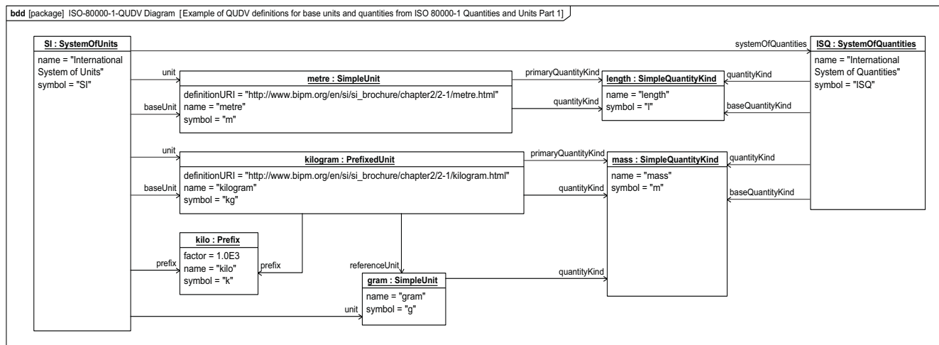
Figure E.8 - Base Unit and Quantity Kinds of the SI and ISQ respectively
