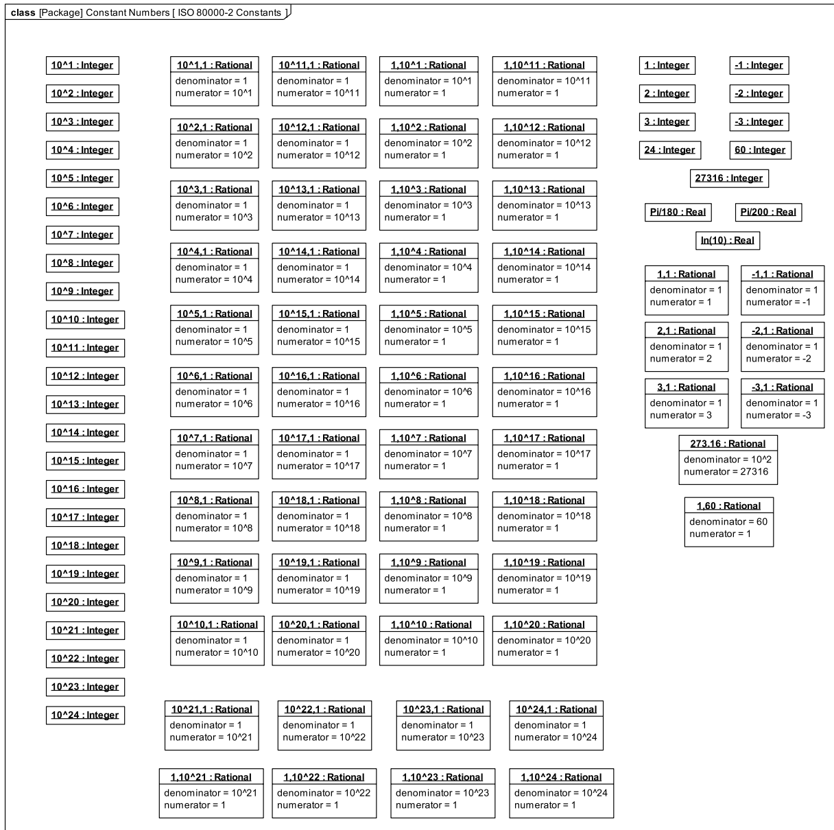
Figure E.19 - Constant numbers used throughout the SysML ISO 80000 library.
