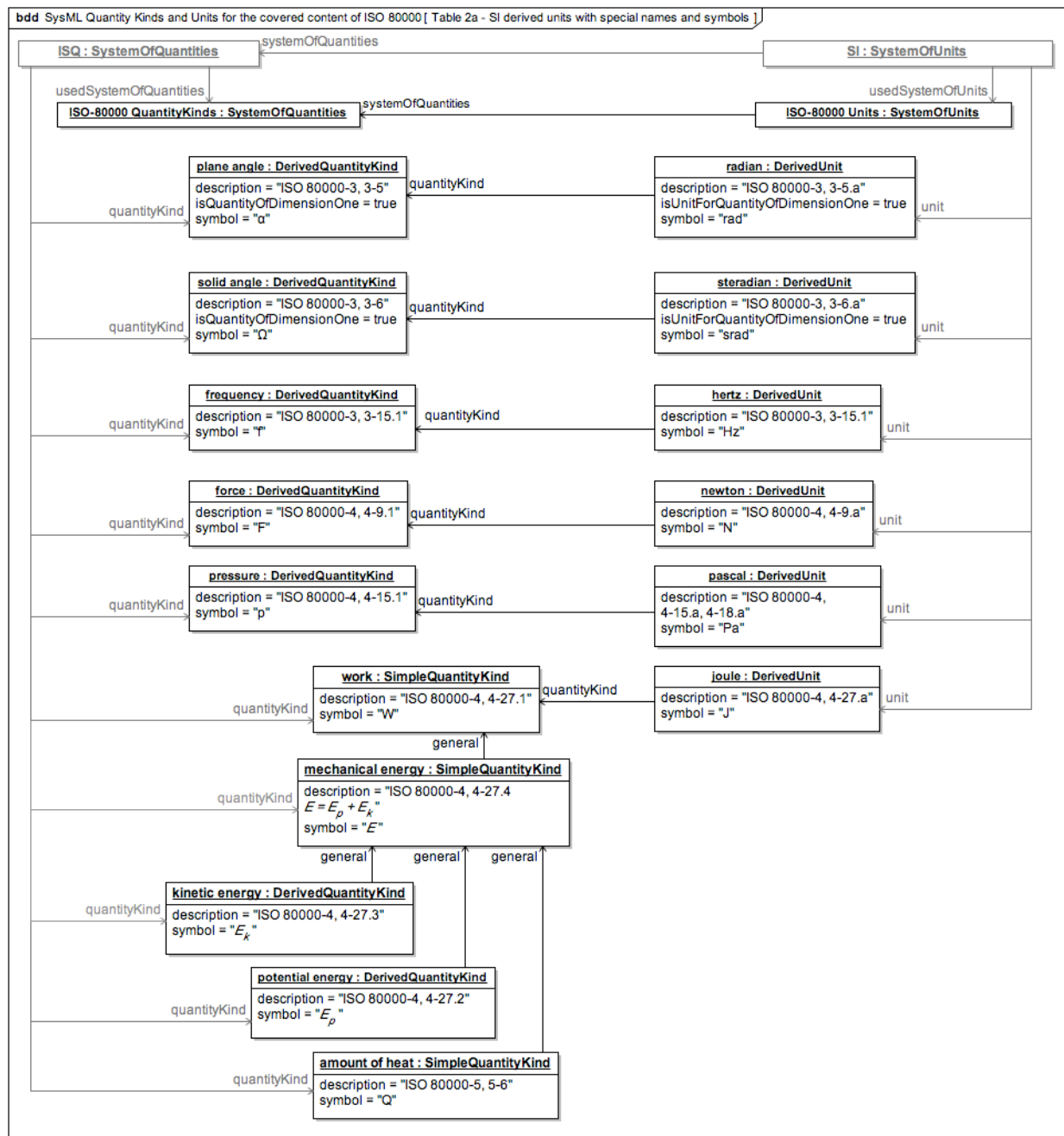
Figure E.15 - Table 2 (from ISO 80000-1) ISQ derived quantities and SI derived units with special names (1)
