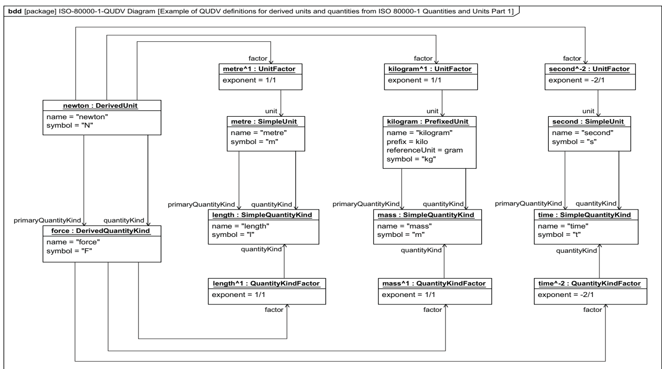
Figure E.9 - Example of a derived unit and derived quantity kind
