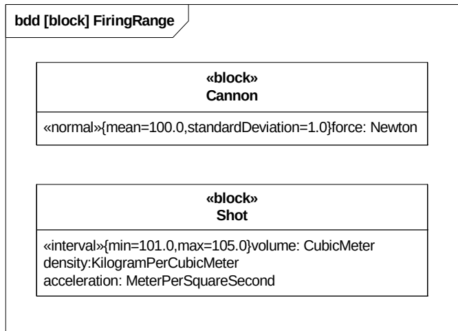
Figure E.21 - Distribution Example
