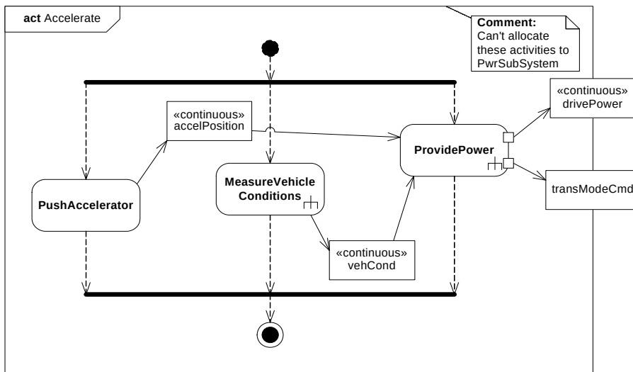
Figure D.36 - Behavior Model for "Accelerate" Function (Activity Diagram)
