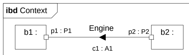
Figure 9.16 - Usage example of item flow decomposition
