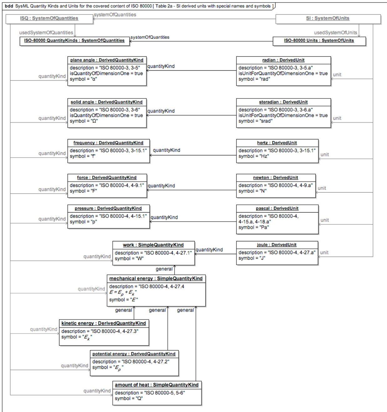
Figure E.14 - Table 2 (from ISO 80000-1) ISQ derived quantities and SI derived units with special names (1)
