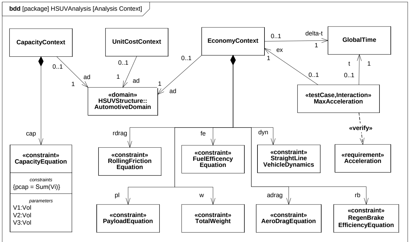
Figure D.26 - Defining Analyses for Hybrid SUV Engineering Development (Block Definition Diagram)
