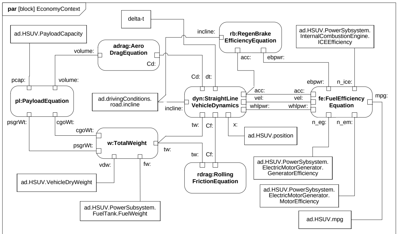
Figure D.32 - Establishing Mathematical Relationships for Fuel Economy Calculations (Parametric Diagram)
