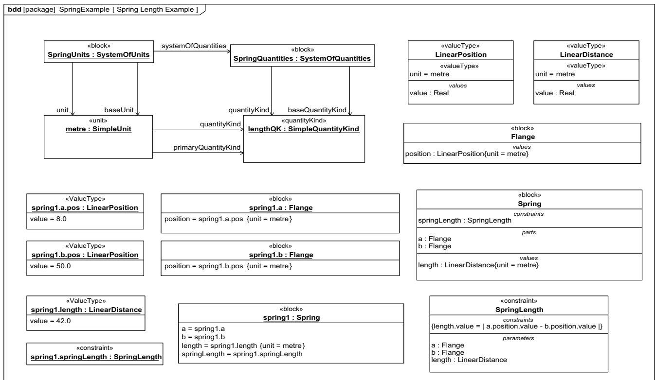
Figure E.9 - Spring Length Example
