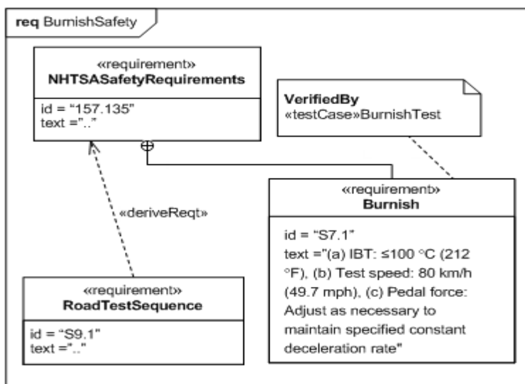
Figure 16.6 - Linkage of a Test Case to a requirement: This figure shows the Requirement Diagram
