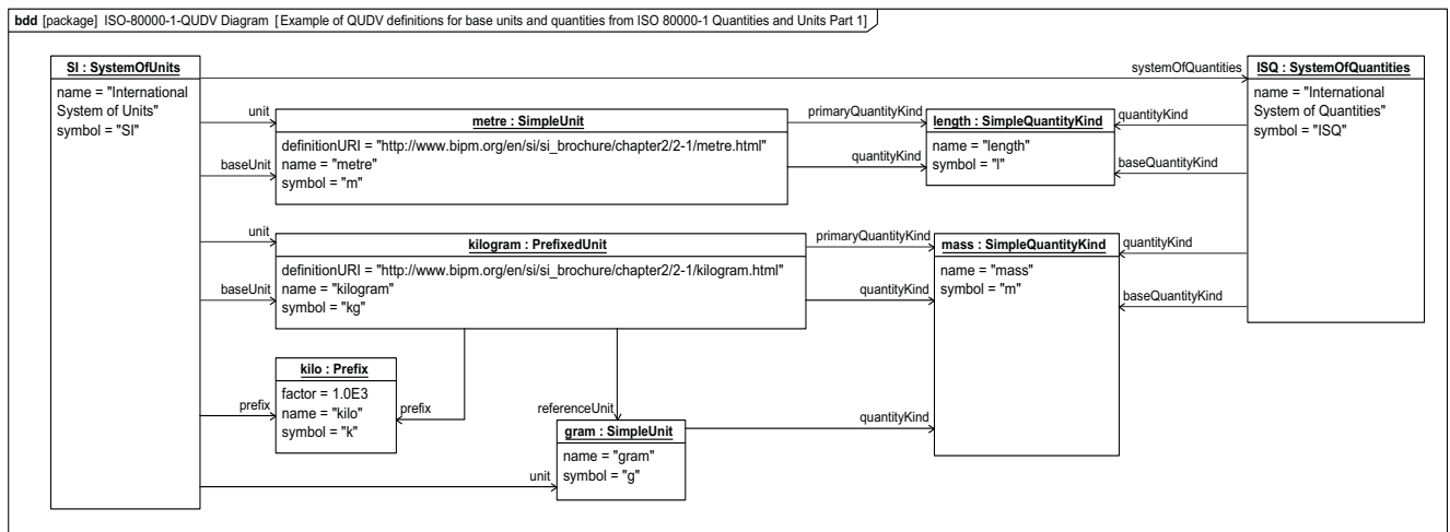
Figure E.7 - Base Unit and Quantity Kinds of the SI and ISQ respectively
