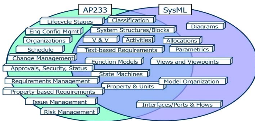
Figure G.1 - SysML/AP233 Data Overlaps
