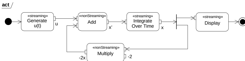
Figure E.2 - Example activity with «streaming» and «nonStreaming» stereotypes applied to subactivities
