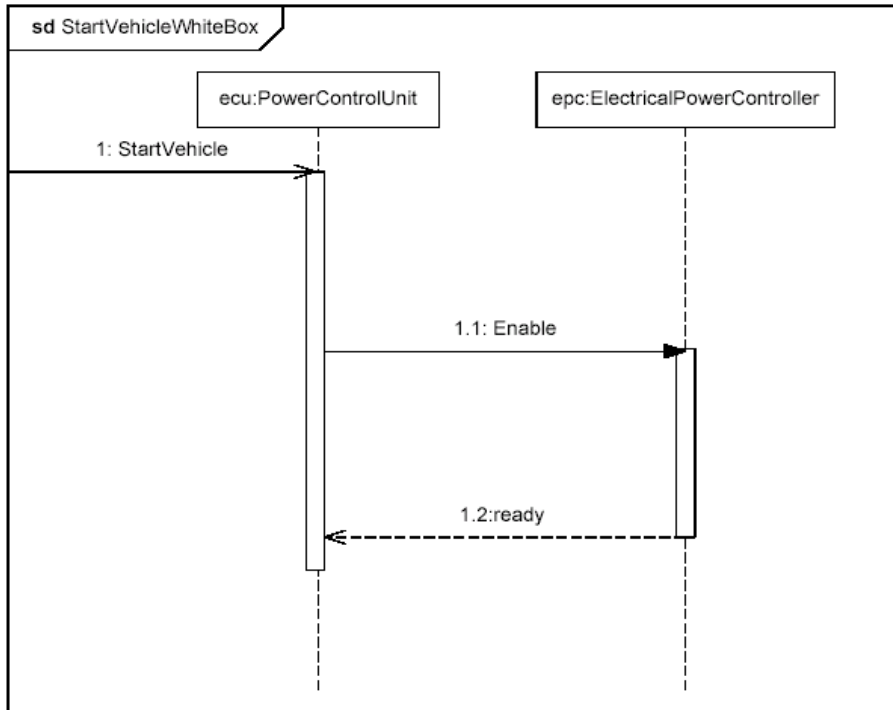
Figure D.10 - White Box Interaction for “StartVehicle” (Sequence Diagram)
