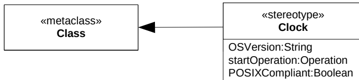
Figure 17.1 - Defining a stereotype
