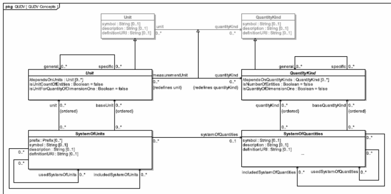
Figure E.4 - QUDV Concepts diagram
