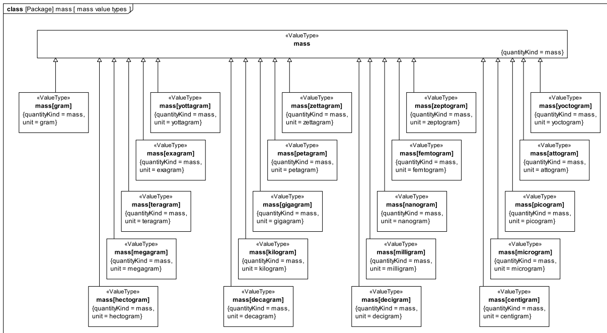
Figure E.19 - Example of value type definitions for a quantity and applicable units and prefixed units
