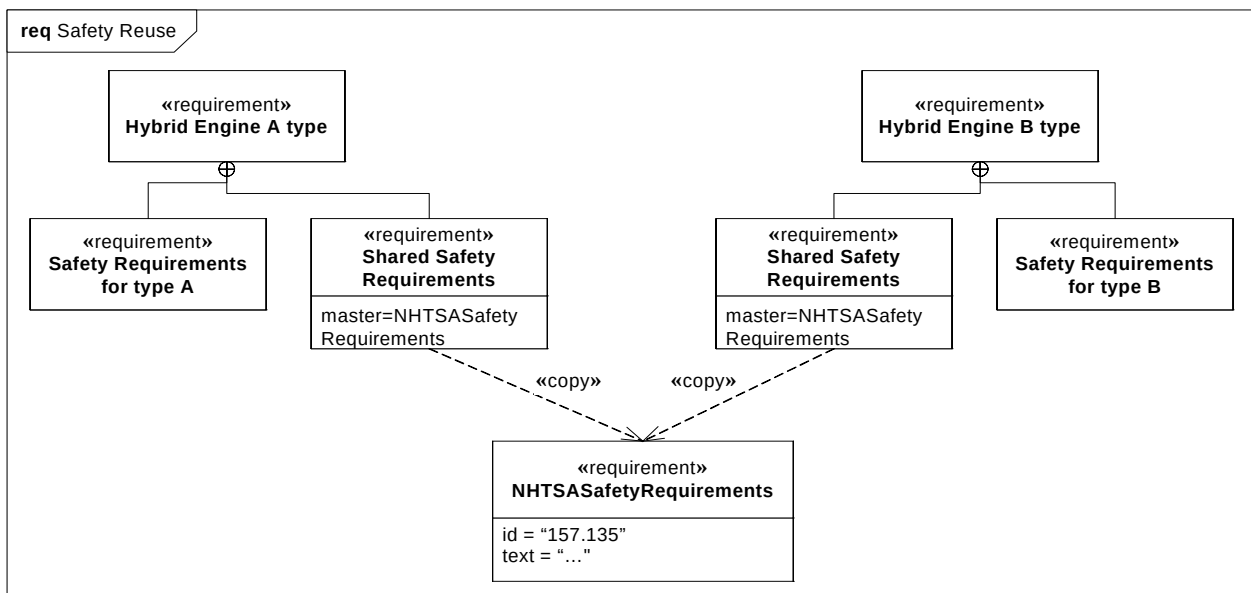
Figure 16.5 - Use of the copy dependency to facilitate reuse
