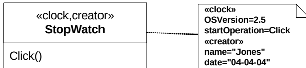
Figure 17.3 - Using stereotypes and showing values
