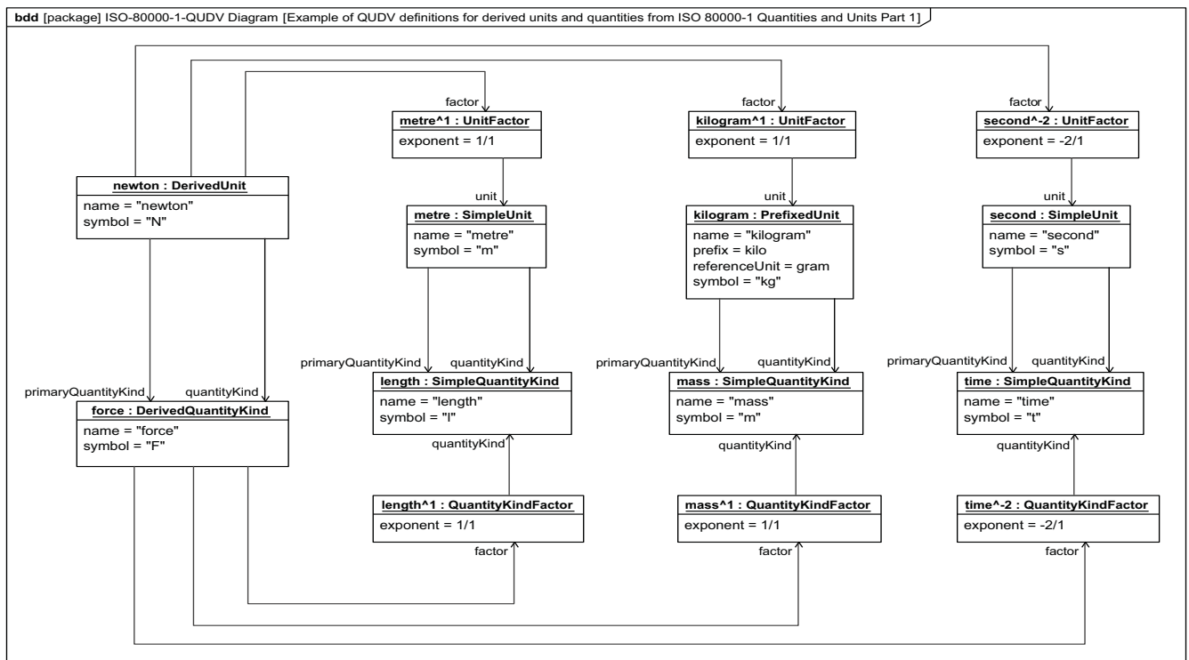
Figure E.8 - Example of a derived unit and derived quantity kind
