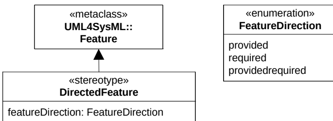
Figure 9.4 - Provided and Required Features
