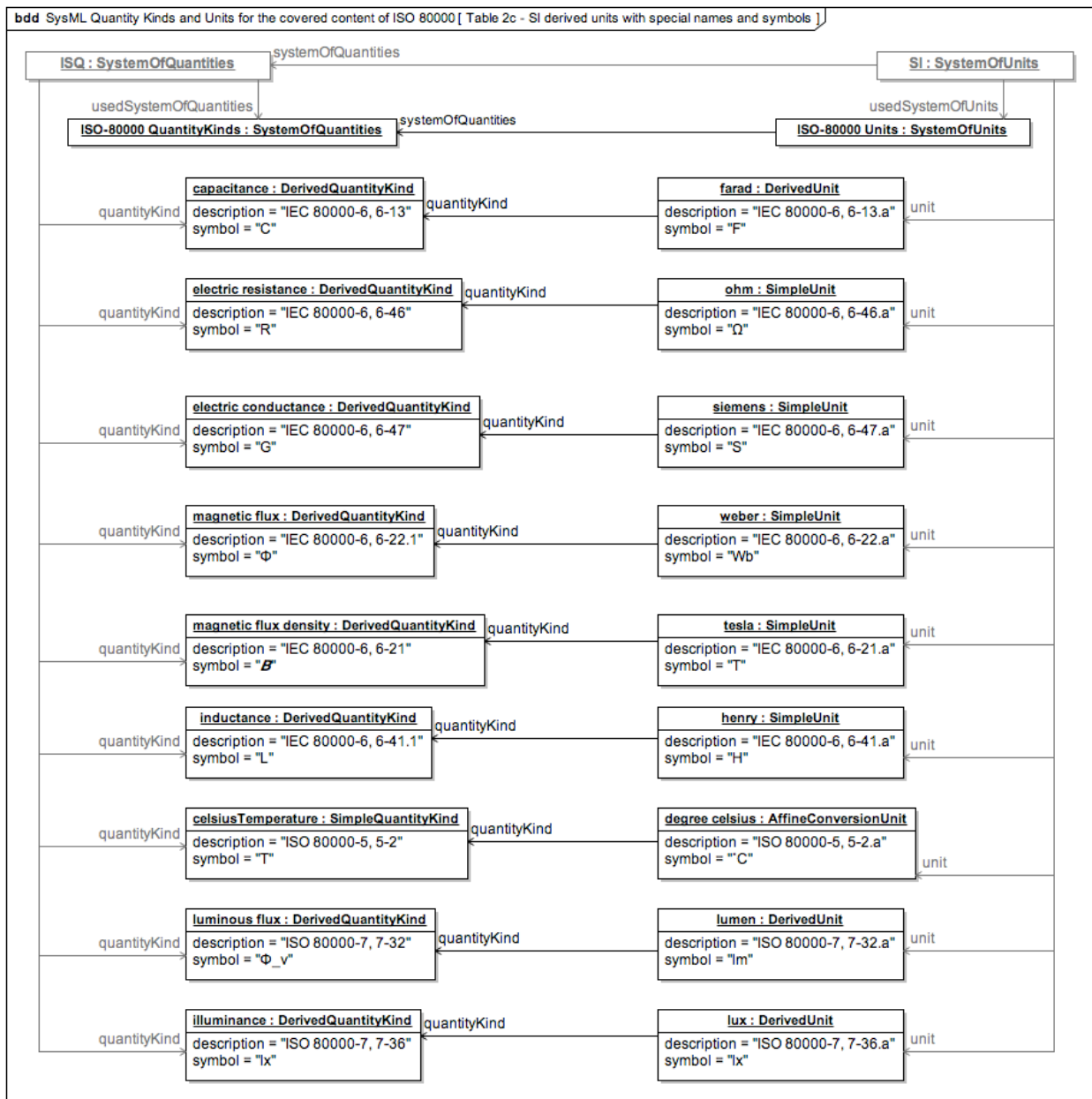
Figure E.16 - Table 2 (from ISO 80000-1) ISQ derived quantities and SI derived units with special names (3)
