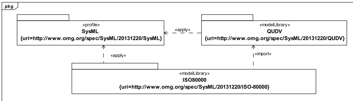
Figure E.10 - Model libraries of SysML Quantity Kinds and Units for the covered content of ISO 80000 parts 3,4,5,6,7,9,10 and 13
