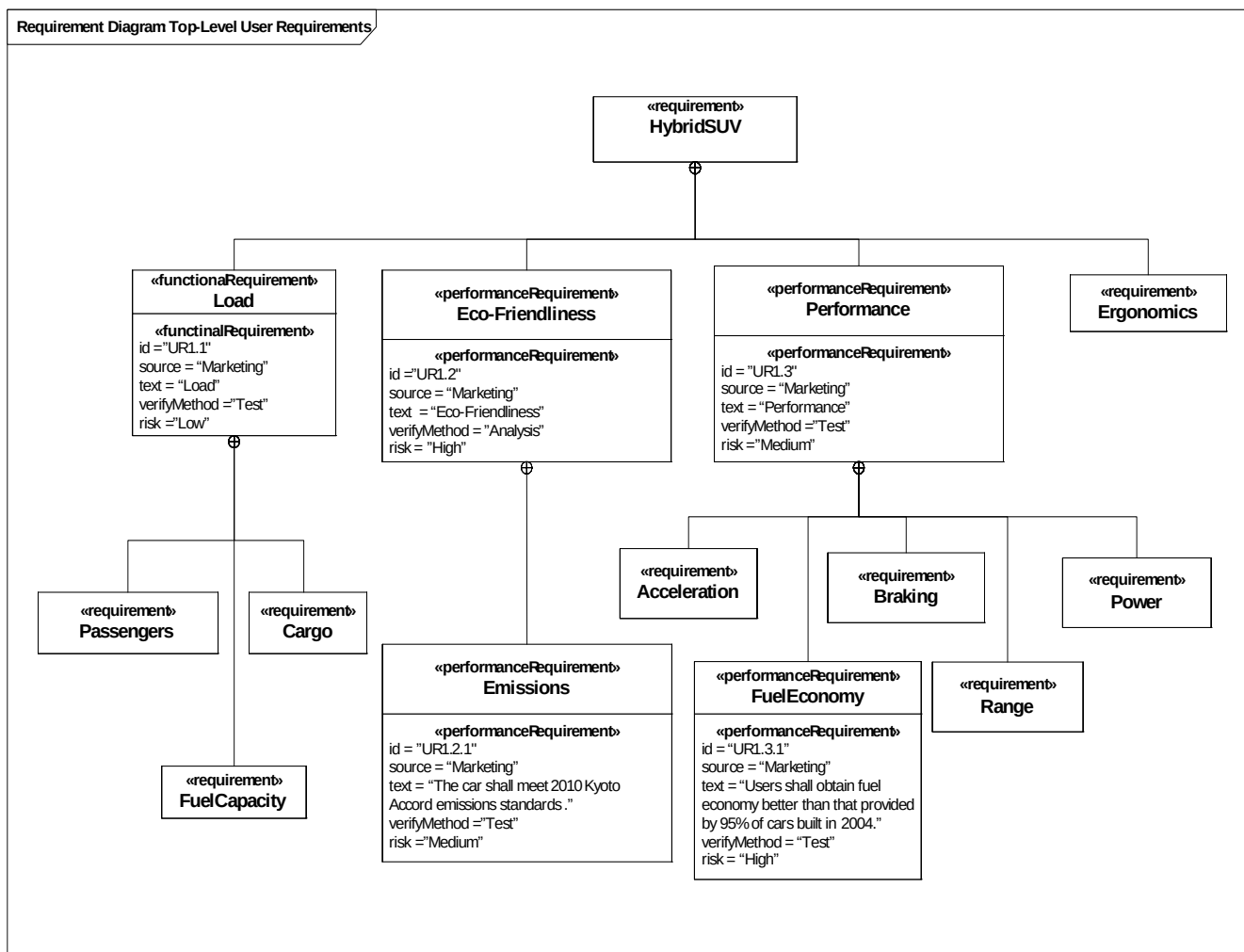
Figure E.3 - Example extensions to Requirement
