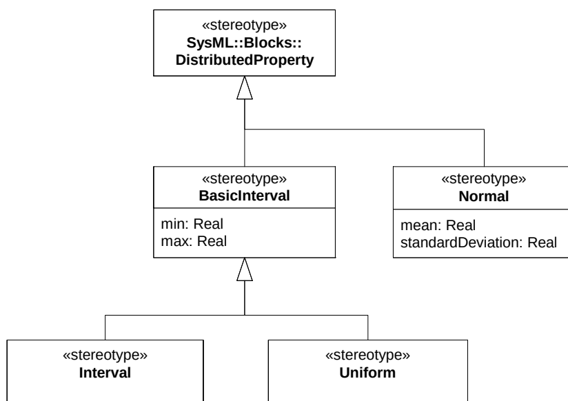
Figure E.20 - Basic distribution stereotypes
