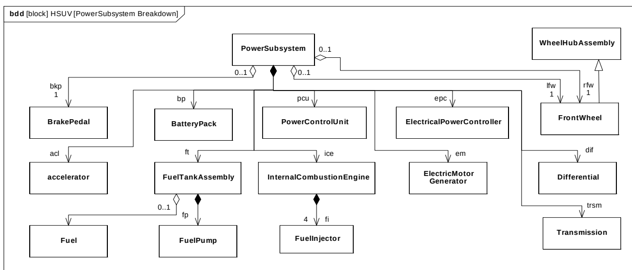
Figure D.18 - Defining Structure of Power Subsystem (Block Definition Diagram)
