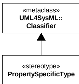
Figure 8.7 - Abstract syntax extensions for SysML property-specific types
