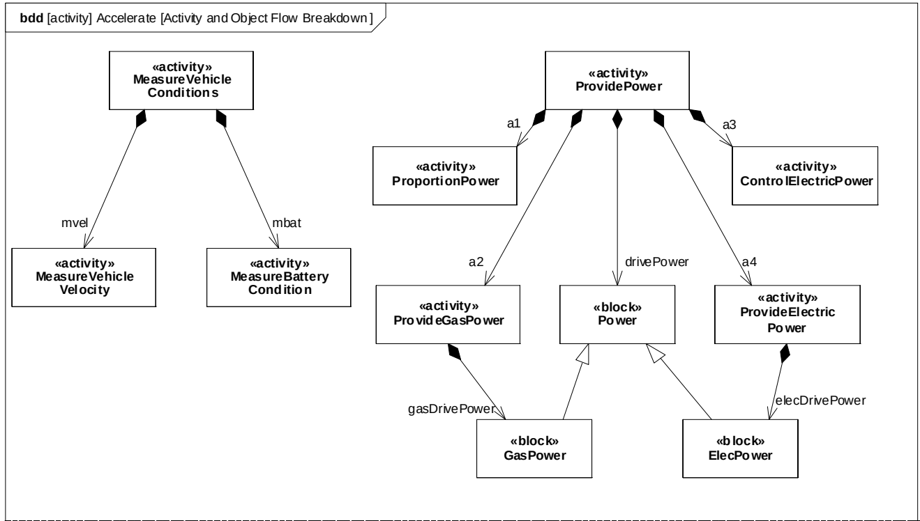
Figure D.37 - Decomposition of “Accelerate” Function (Block Definition diagram)
