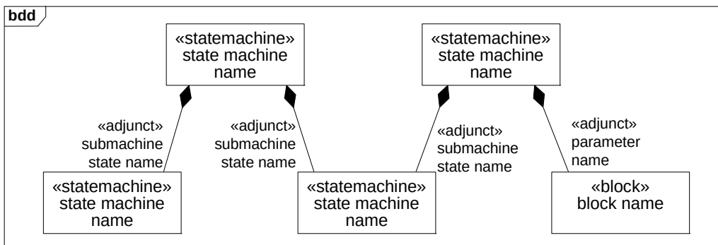
Figure 13.1 - Block definition diagram with state machines as blocks associated with submachines and types of parameters
