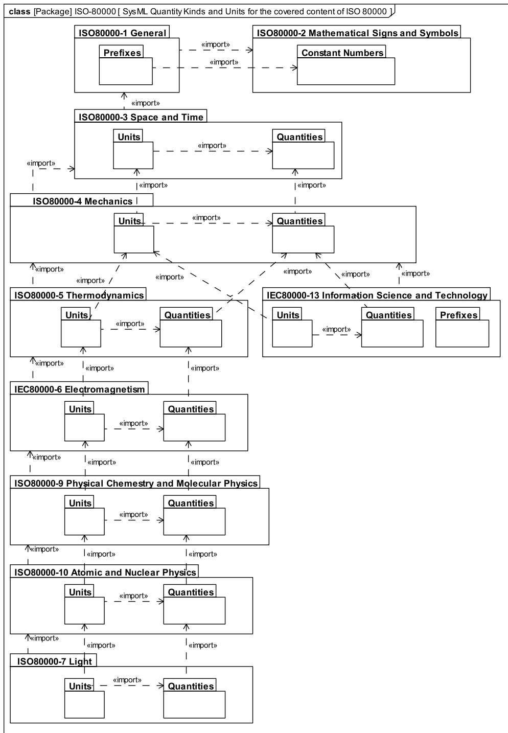
Figure E.11 - Organization of the definitions of units and quantities from the normative parts of ISO 80000 covered in SysML 1.4, which includes all the normative content of parts 3,4,5,6; the subset of parts 7,9,10 corresponding to the content from SysML and the subset of part 13 pertaining to commonly used units of information. Parts 8,11 and 12 are not covered because none of their units and quantities were referenced in previous versions of SysML nor in the summary tables in ISO 80000-1
