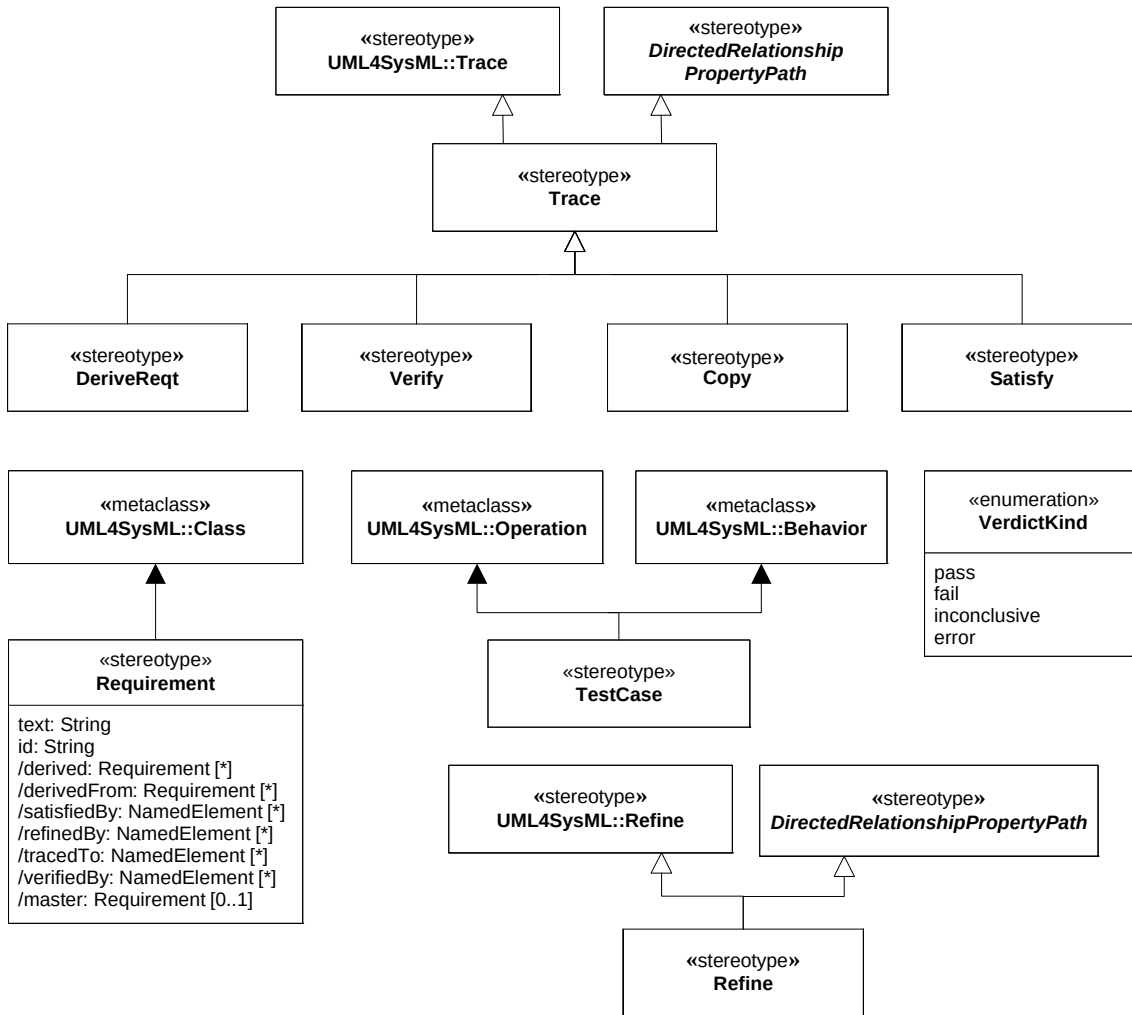
Figure 16.1 - Abstract Syntax for Requirements Stereotypes
