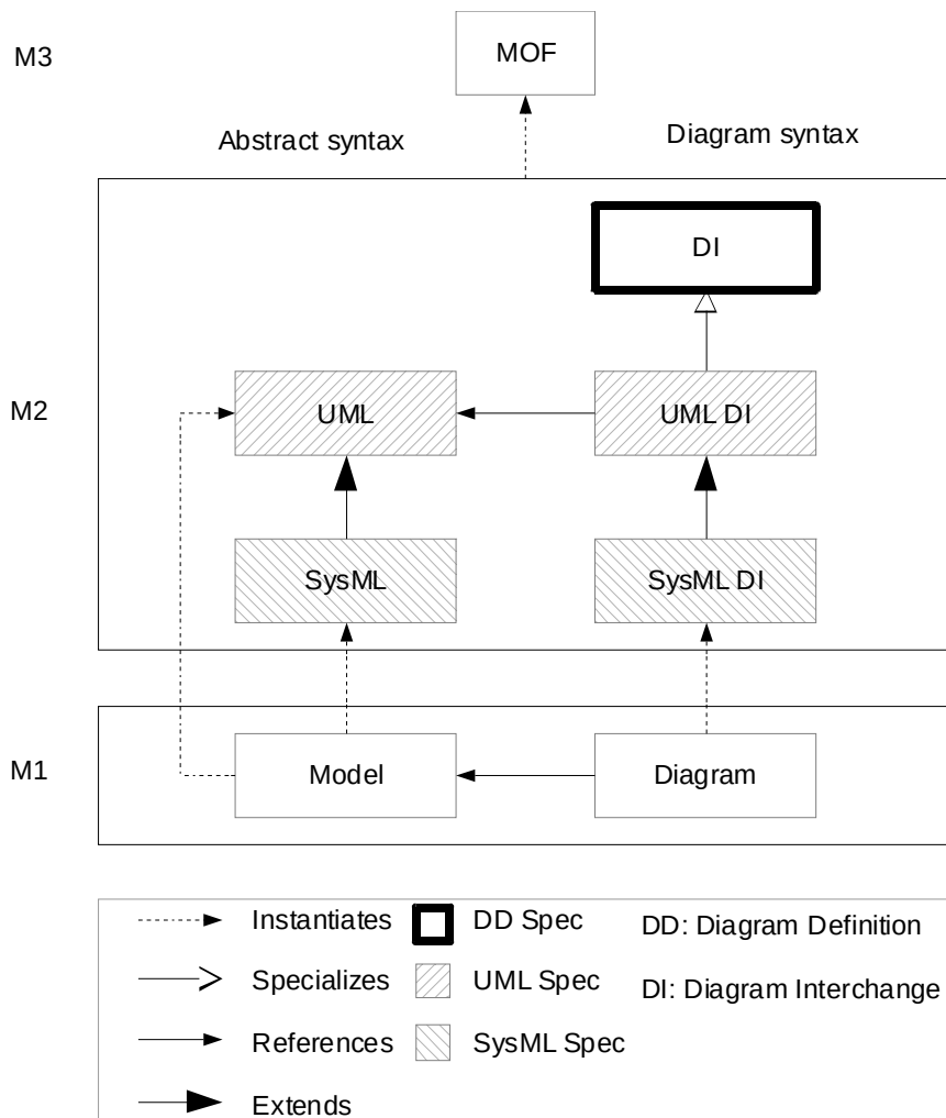
Figure B.1 - SysML DI architecture
