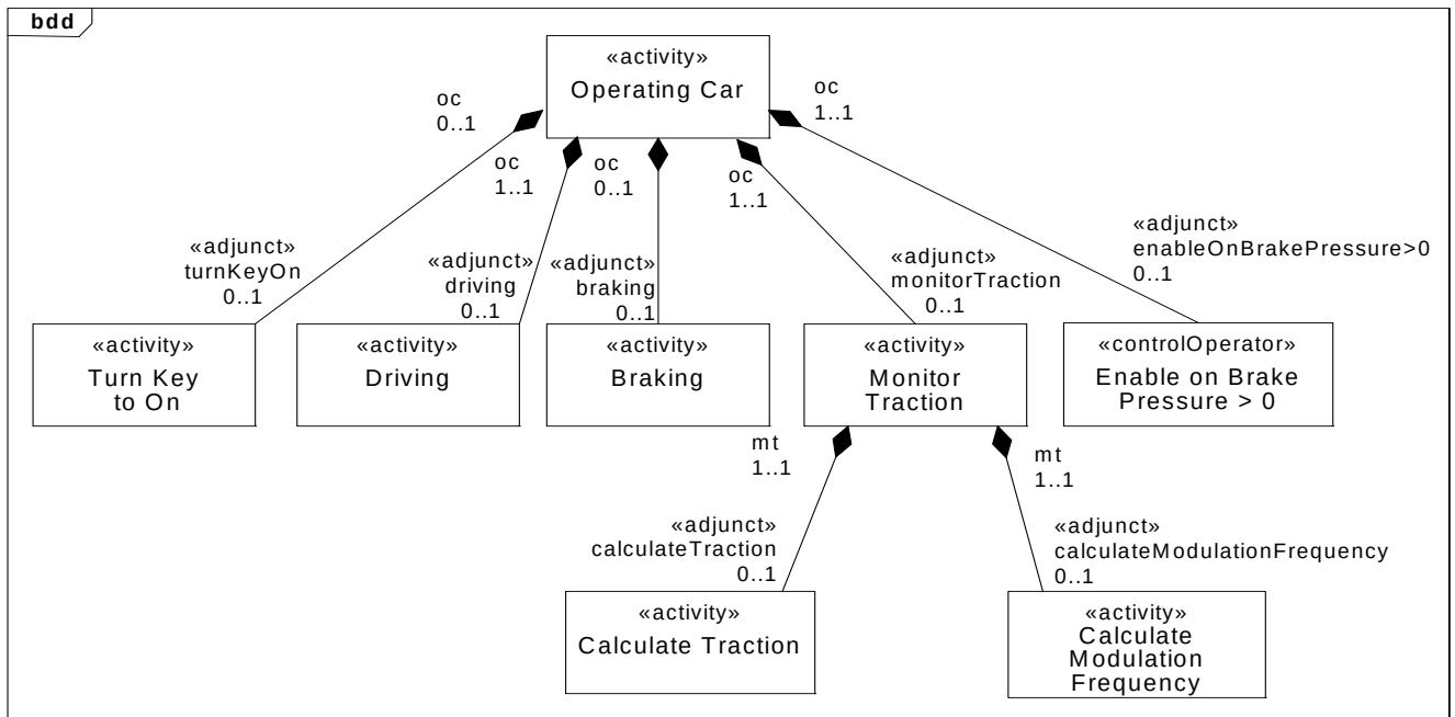
Figure 11.13 - Example block definition diagram for activity decomposition
