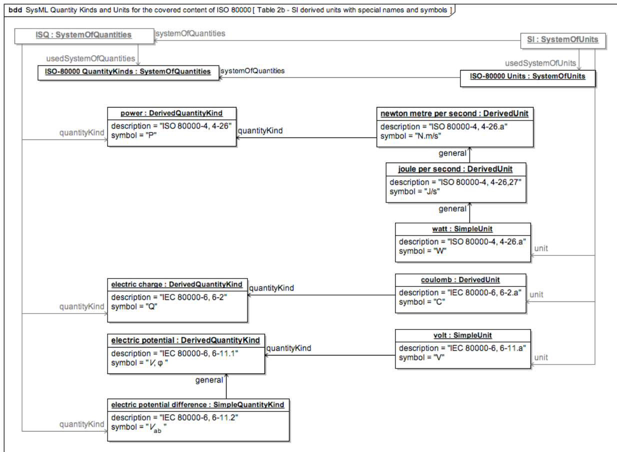
Figure E.15 - Table 2 (from ISO 80000-1) ISQ derived quantities and SI derived units with special names (2)
