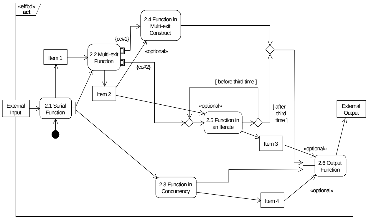
Figure E.1 - Example activity with «effbd» stereotype applied
