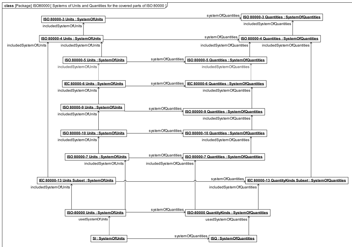
Figure E.12 - Content relationships for the systems of units and quantities in from the different parts of ISO 80000 in relation to ISO 80000 as a whole and to the International System of Units (SI) and quantities (ISQ)
