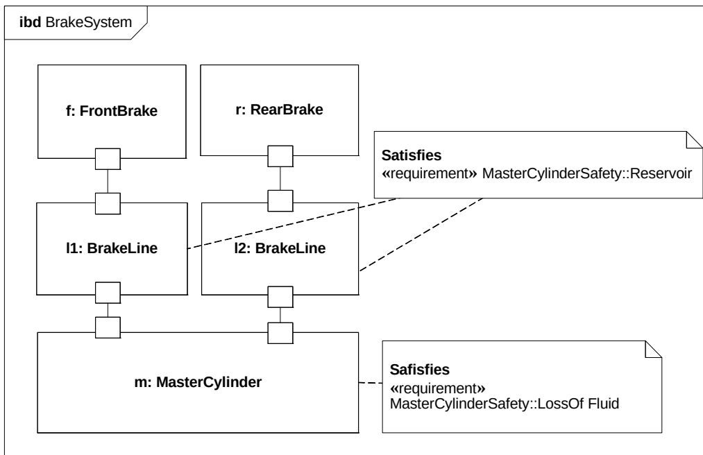
Figure 16.4 - Requirement satisfaction in an internal block diagram
