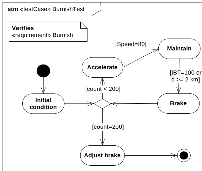
Figure 16.7 - Linkage of a Test Case to a requirement: This figure shows the Test Case as a State Diagram
