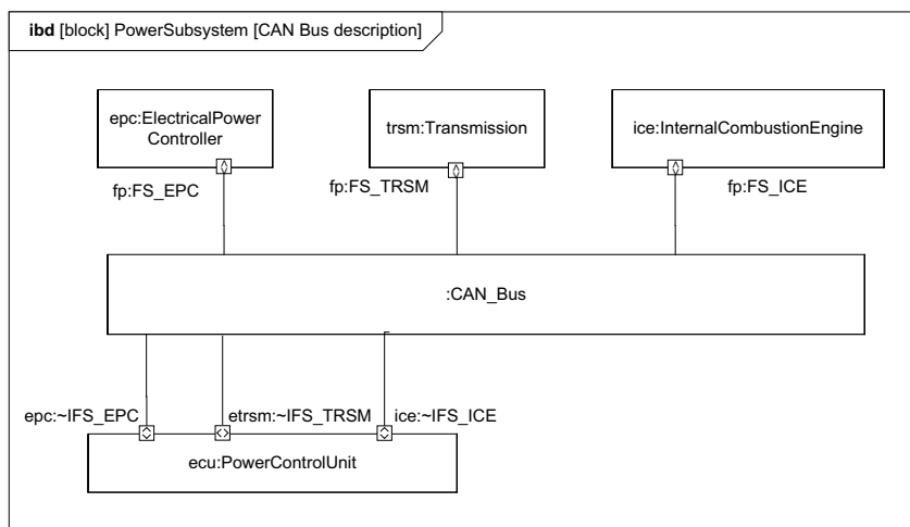
Figure D.22 - Consolidating Connectors into the CAN Bus. (Internal Block Diagram)
