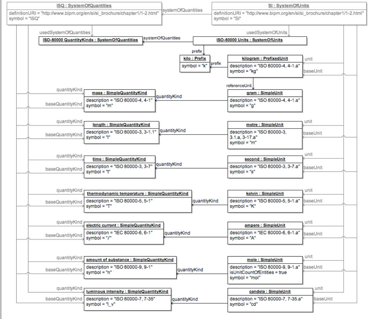
Figure E.13 - Table 1 (from ISO 80000-1) SI base units for the ISQ base quantities
