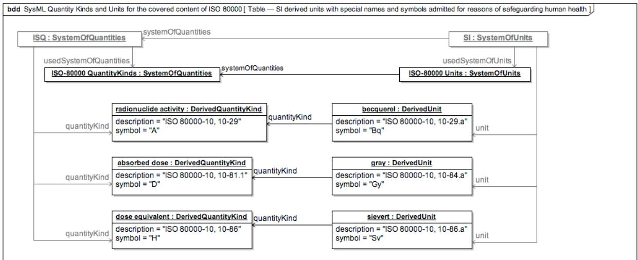
Figure E.17 - Table 3 (from the SI brochure) SI derived units with special names and symbols
