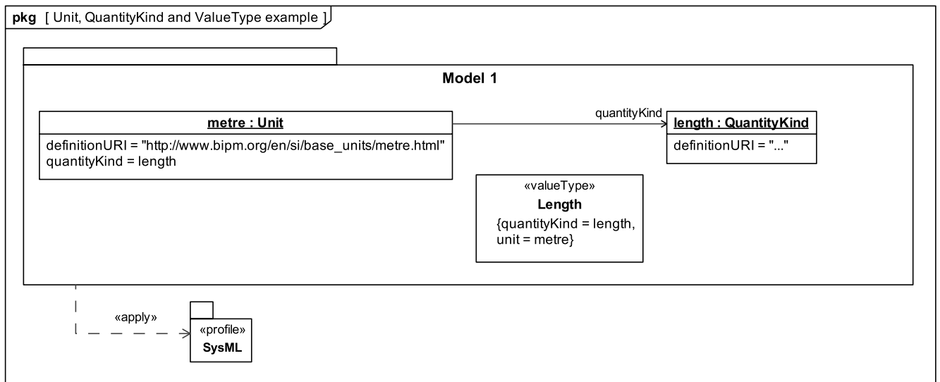
Figure 8.18 - Example of Unit, QuantityKind and ValueType definitions
