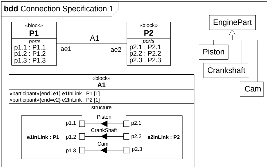
Figure 9.16 - Usage example of item flow decomposition
