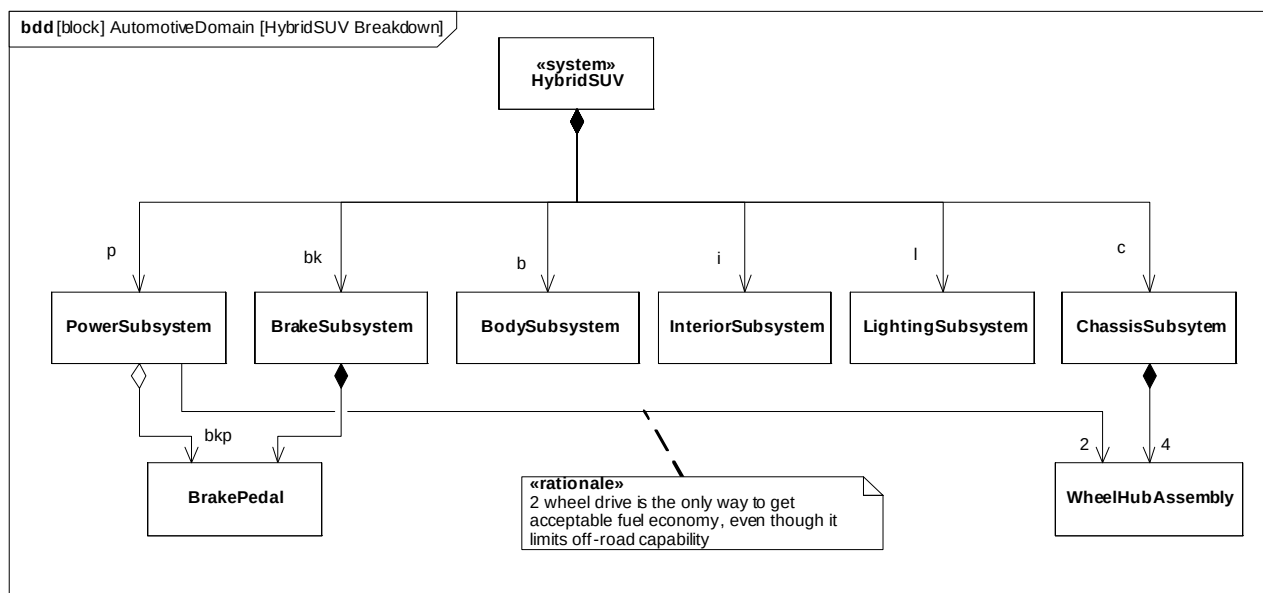
Figure D.16 - Defining Structure of the Hybrid SUV System (Block Definition Diagram)
