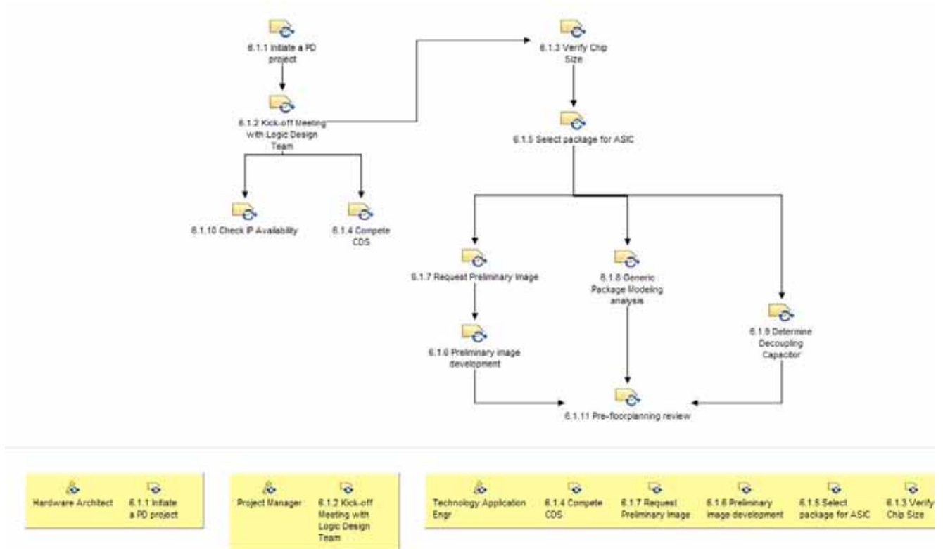
Figure C.22 - A workflow in the ASIC method (top) defining control flow amongst task uses as well as list of the same task uses grouped by performing role
