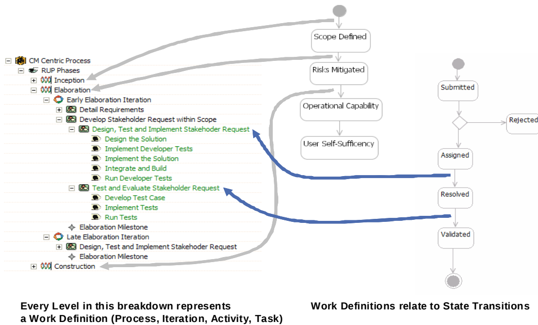
Figure 7.9 - Another view of how state transitions relate to work definitions
