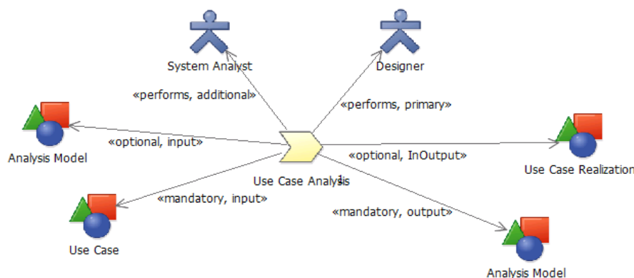
Figure 7.2 - The same SPEM 2.0 class diagram of Figure 7-1 using SPEM 1.1 stereotype icons
