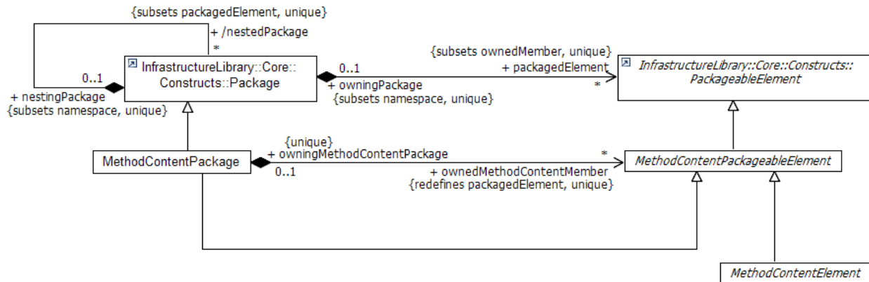
Figure 13.6 - ContentPackage redefines its inherited owned Members association to only allow Method Content Elements
