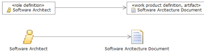
Figure 12.4 - Example for a UML2 diagram with role stereotypes and artifact responsibility
