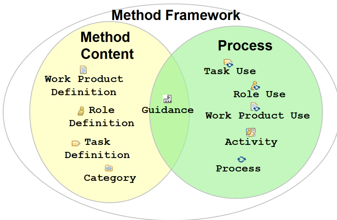
Figure 6.5 - Key terminology defined in this specification mapped to Method Content versus Process
