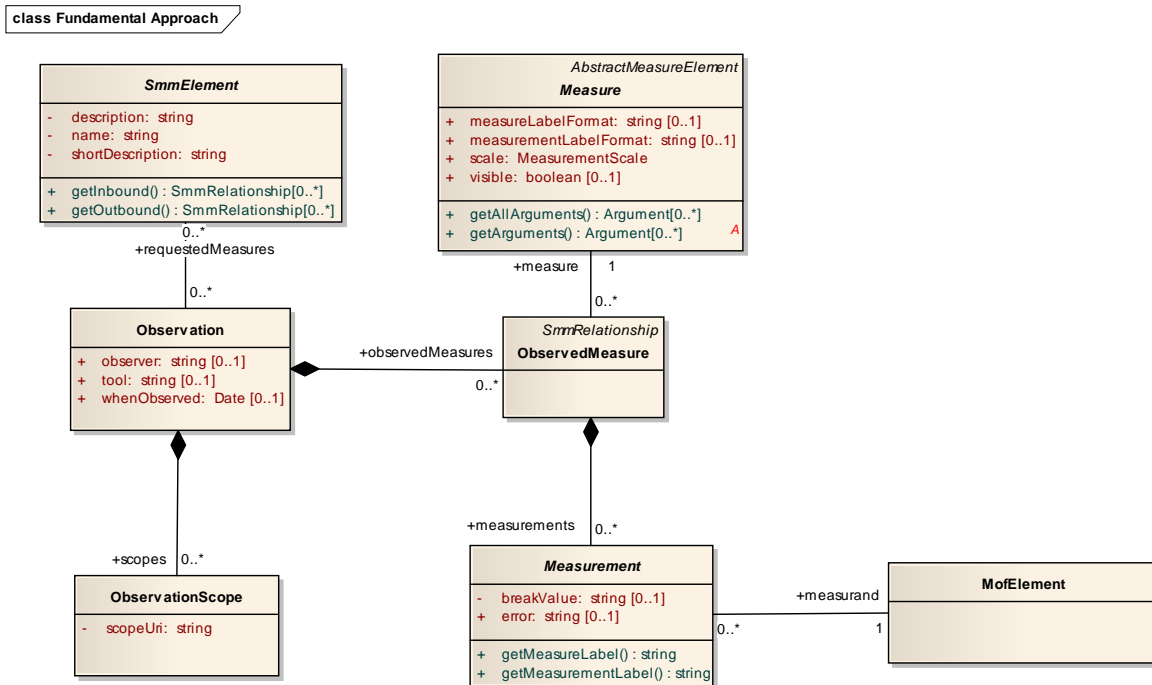
Figure 7.1 - Fundamental Approach
