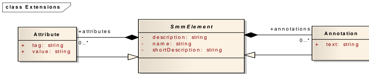
Figure 9.1 - SMM Extensions
