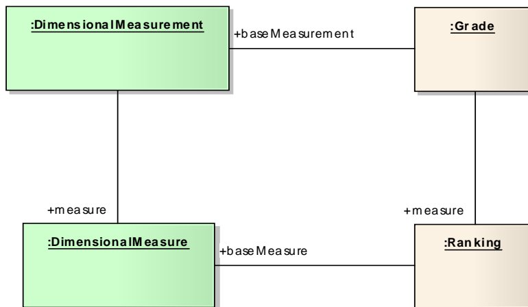
uc GradeConstraint
