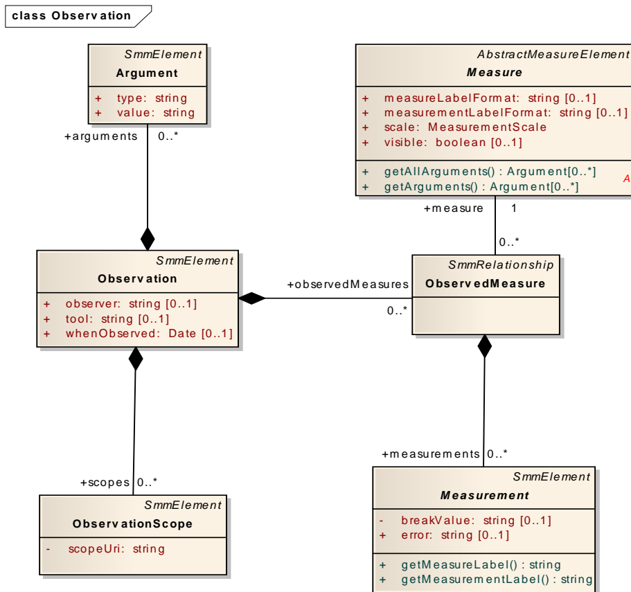
Figure 16.1 - Observations
