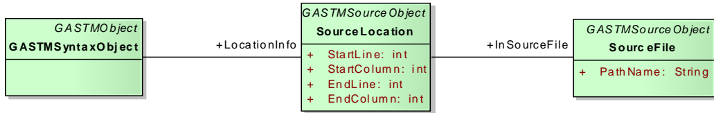
Figure 19.14 - GASTM Fragment
