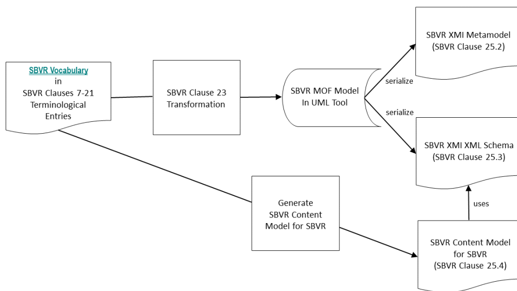
Figure 23.1 - SBVR Machine-Readable File Transformation
