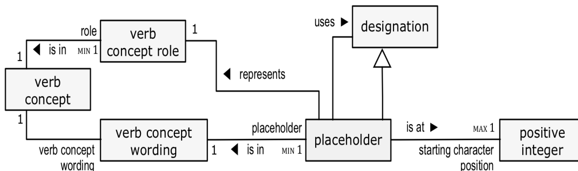
Figure 12.10 - Placeholders in Verb Concept Wordings
