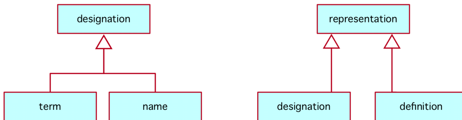
Figure C.16 - Depicting mutually-exclusive categories (diagram on the left) vs. independent specializations (diagram on the right)
