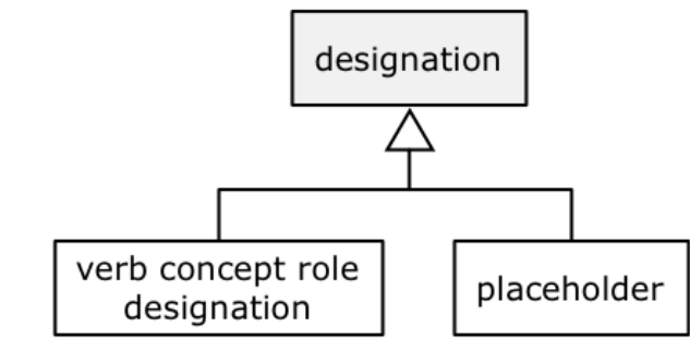
Figure 12.7 - Placeholder and Verb Concept Role Designation
