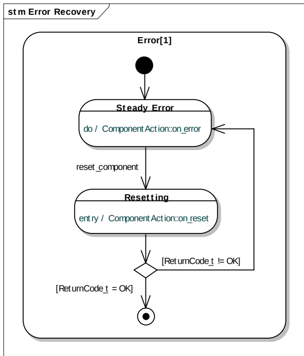
Figure 5.7 - Error Recovery
