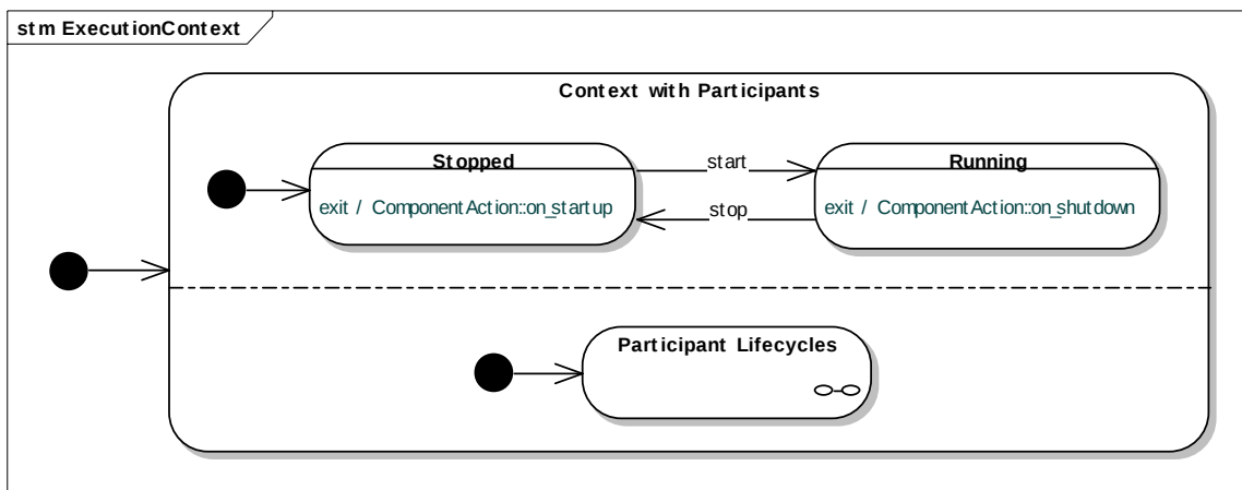
Figure 5.8 - ExecutionContext
