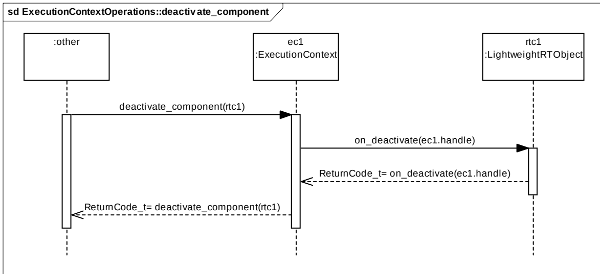
Figure 5.14 - ExecutionContextOperations::deactivate_component
