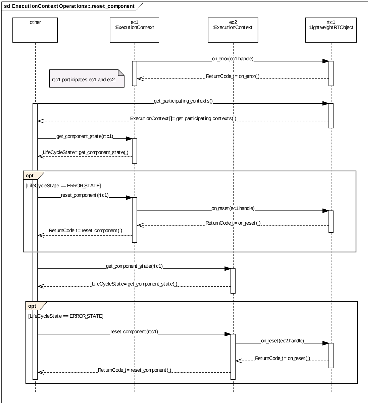
Figure 5.15 - ExecutionContextOperations::reset_component
