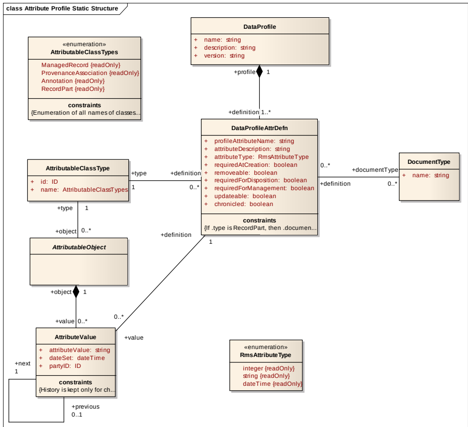
Attribute Profile Static Structure
