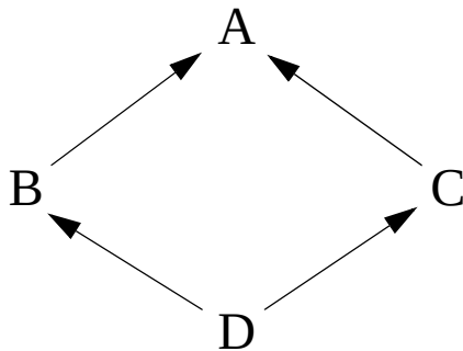
Figure 7.1 - Diamond inheritance hierarchy
