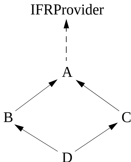
Figure 7.2 - Diamond inheritance hierarchy with implied reflection provider inheritance
