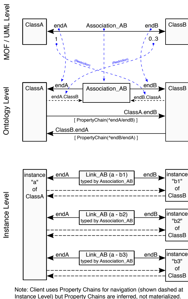
Figure 9.2: MOF Association Transformation Scheme
