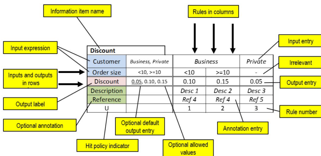
Figure 8-1: Decision table example (vertical orientations: rules as columns)
