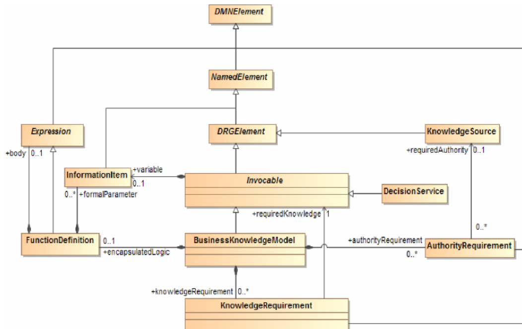
Figure 6-14: BusinessKnowledgeModel class diagram
