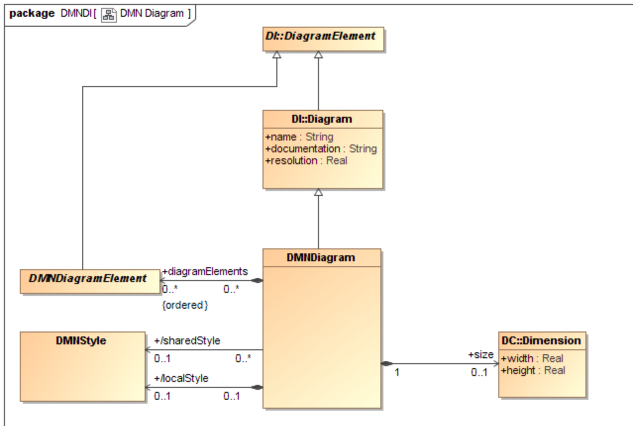
Figure 13-2: DMNDiagram
