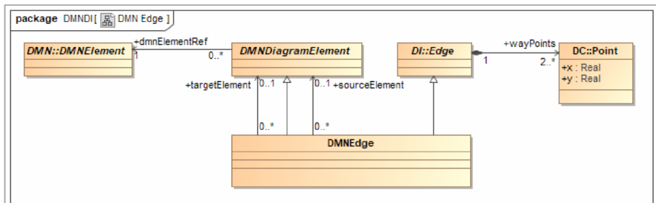
Figure 13-5: DMNEdge
