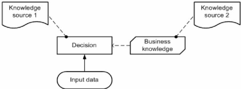
Figure 5-4: Knowledge sources
