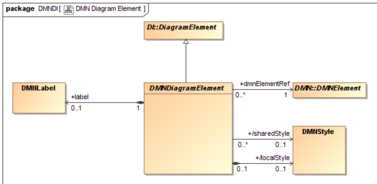
Figure 13-3: DMNDiagramElement
