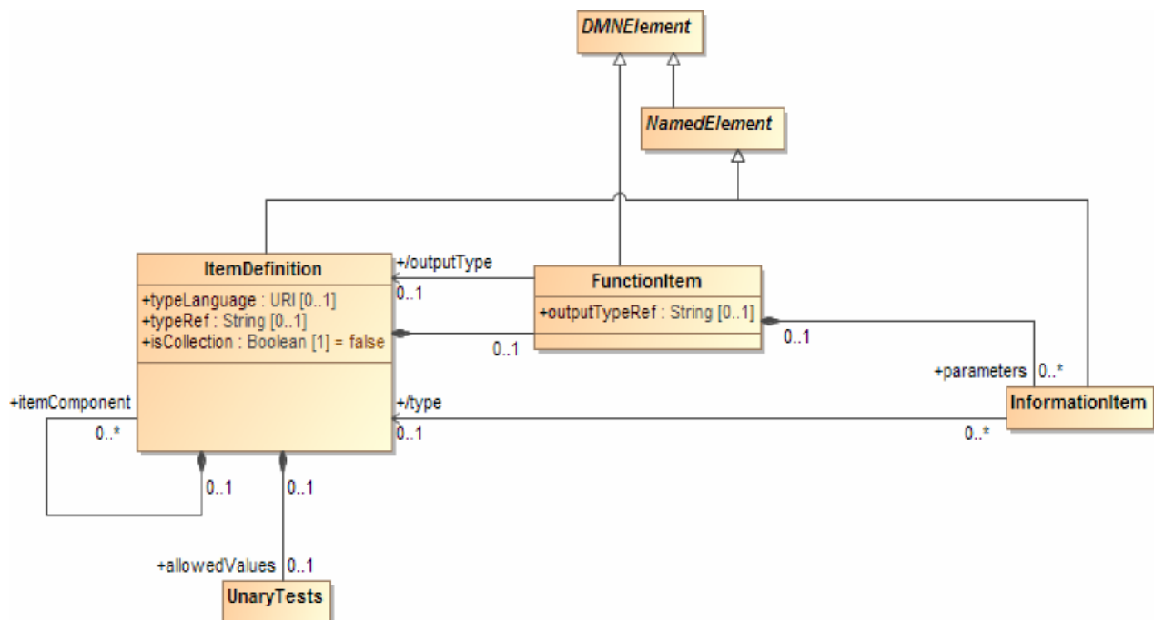
Figure 7-7: ItemDefinition class diagram
