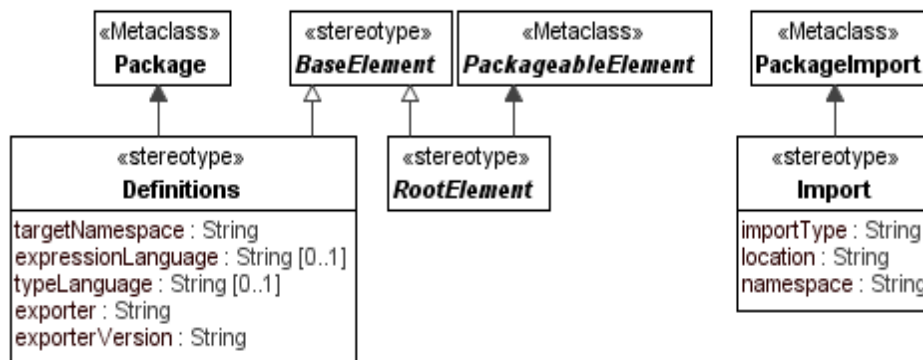
Figure 9.2 - Definitions
