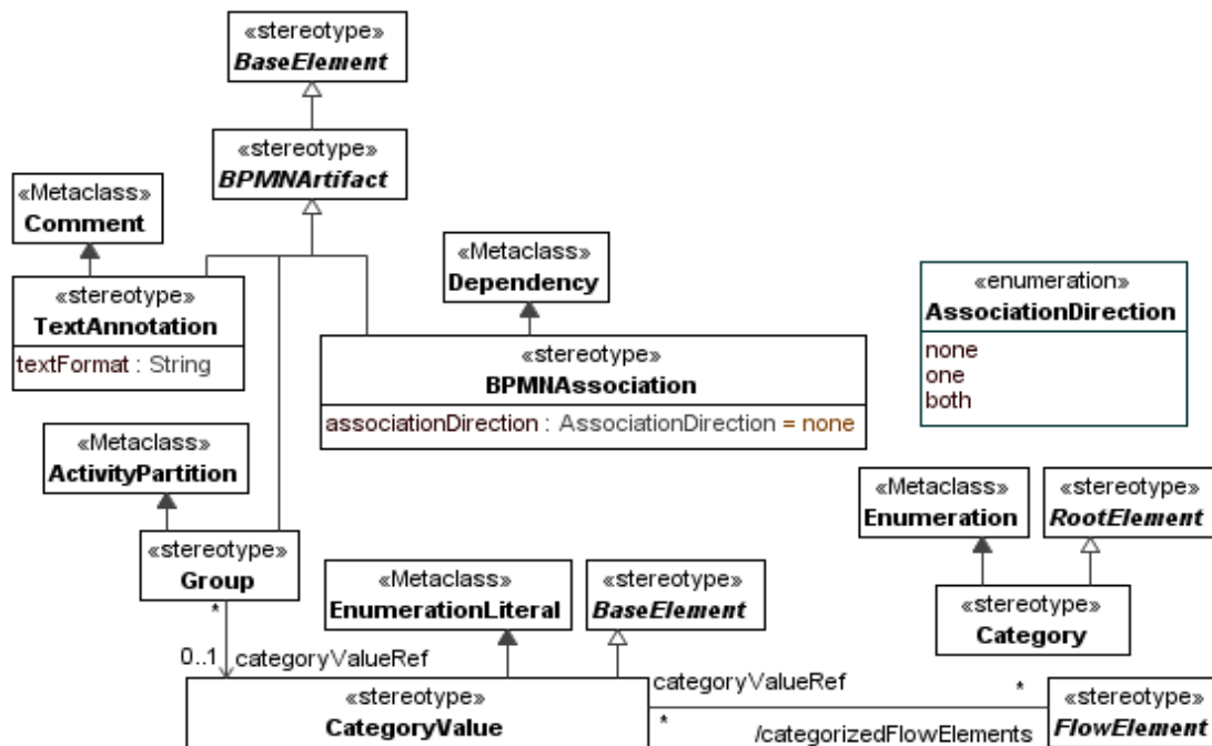
Figure 9.7 - Artifacts
