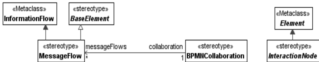
Figure 11.3 - Message Flows
