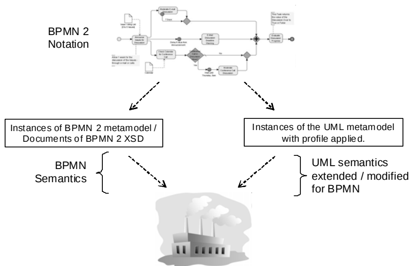
Figure 1.1 - Equivalent Semantics
