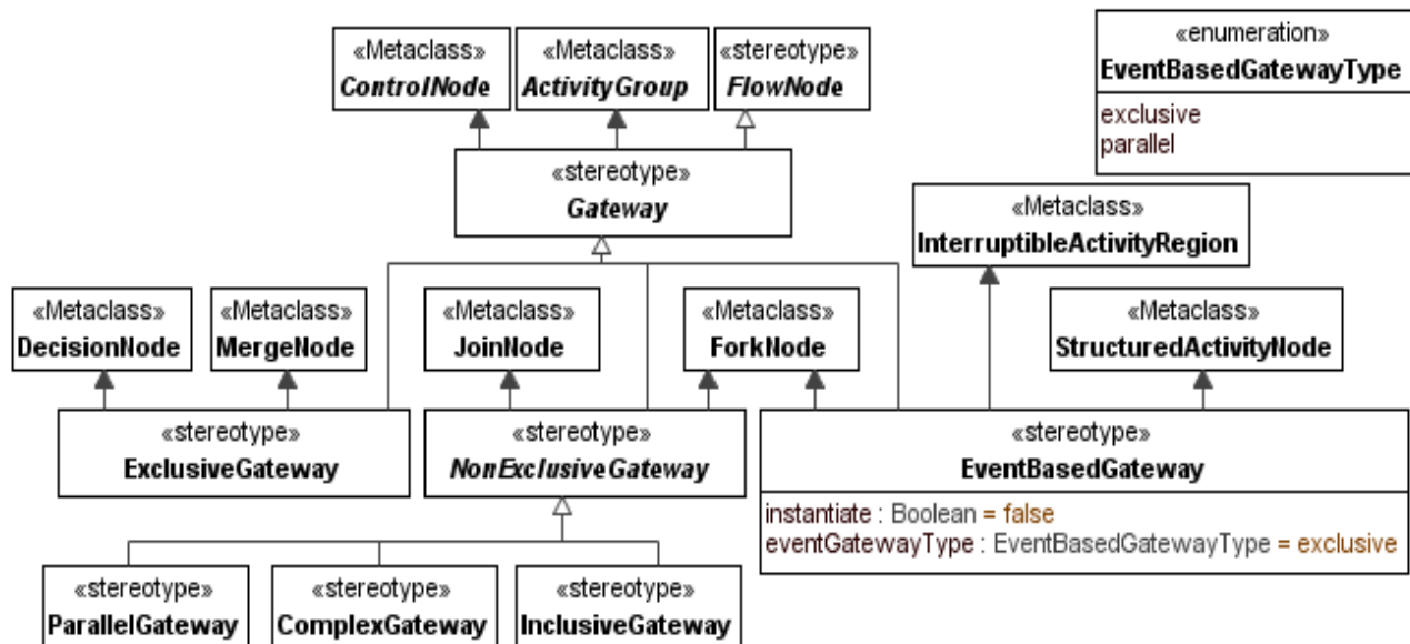
Figure 10.11 - Gateways
