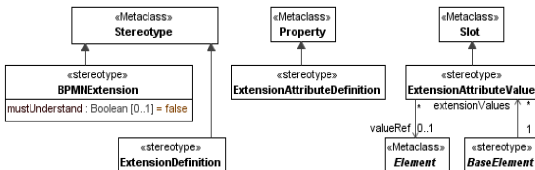
Figure 9.3 - BPMN Extensions
