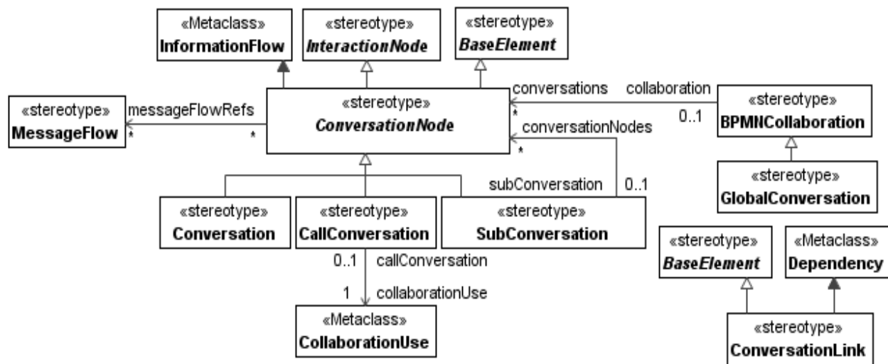
Figure 11.4 - Conversations
