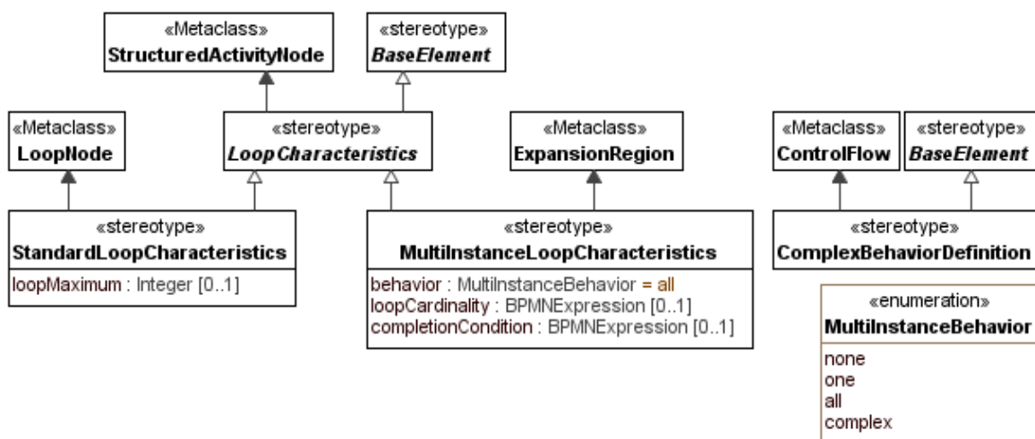
Figure 10.17 - Loop Characteristics
