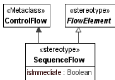
Figure 10.4 - Sequence Flows
