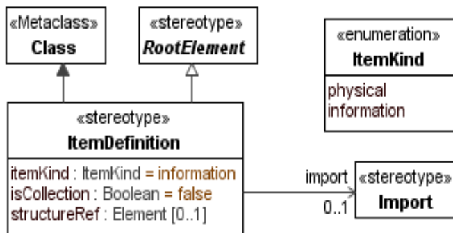
Figure 9.6 - Item Definitions
