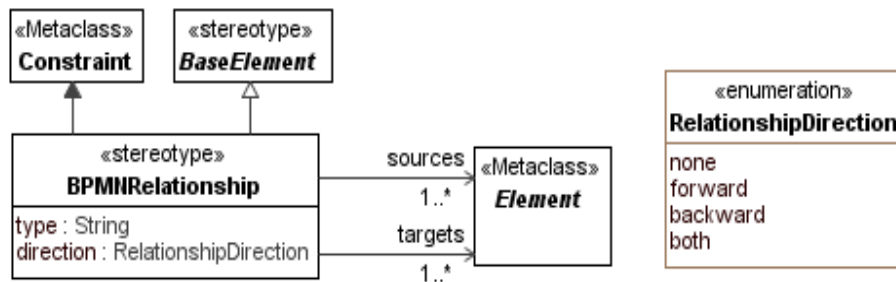
Figure 9.4 - External Relationships
