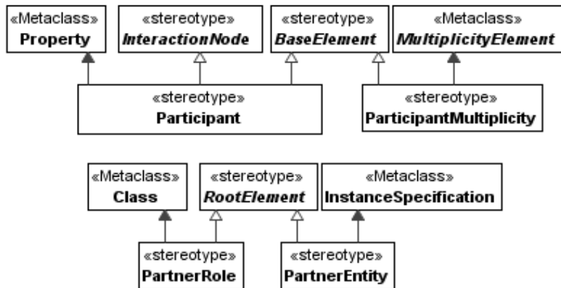
Figure 11.2 - Participants
