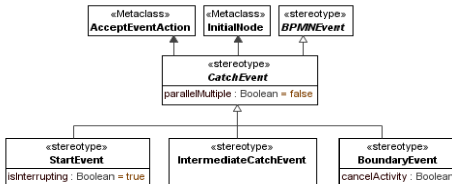
Figure 10.10 - Catch Events
