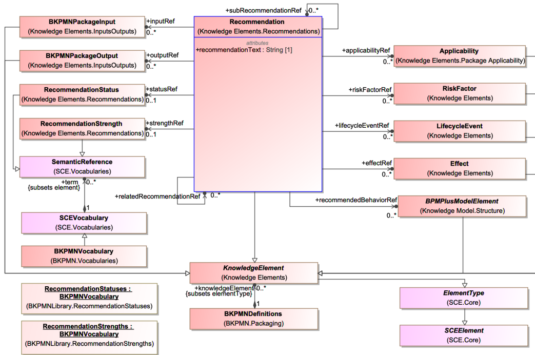
Figure 21: The Recommendations Metamodel
