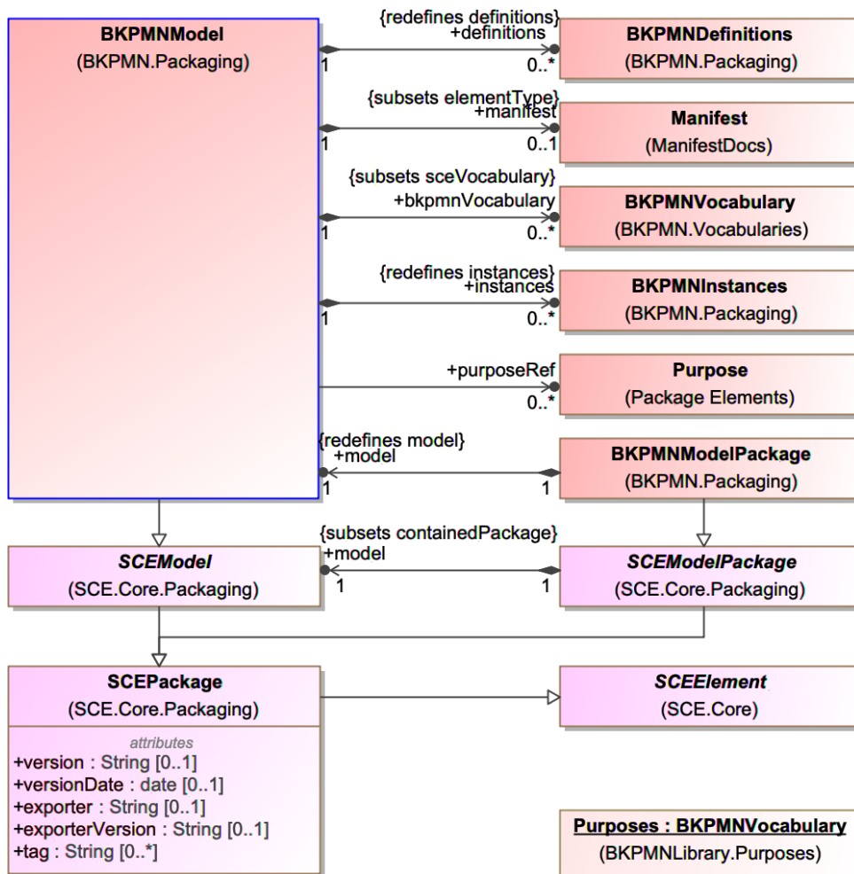
Figure 8: The BKPMNModel Metamodel
