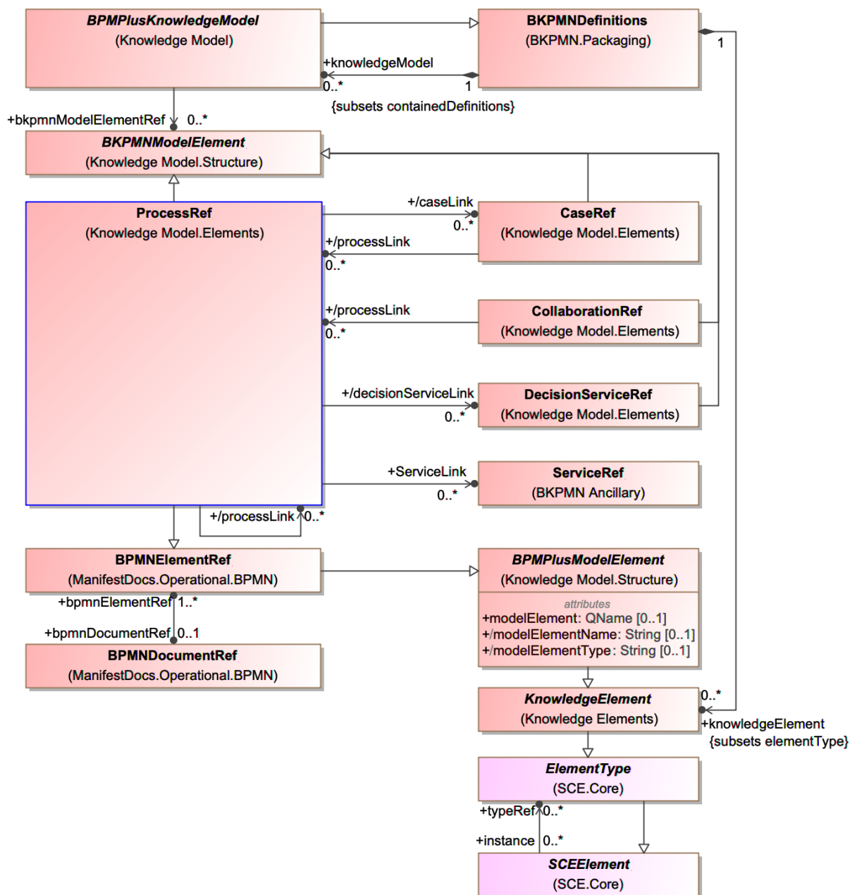
Figure 58: The ProcessRef Metamodel
