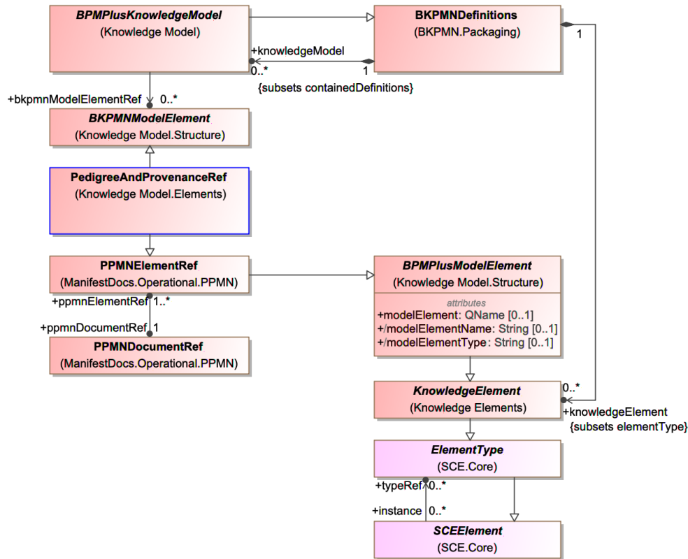
Figure 60: PedigreeAndProvenanceRefMM
