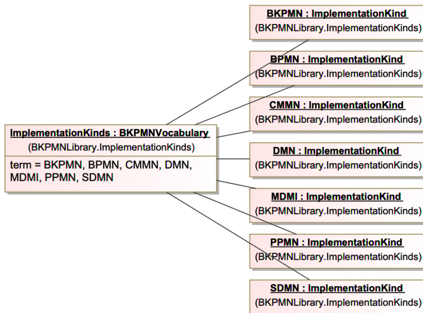
Figure 68: The ImplementationKinds Instance Model
