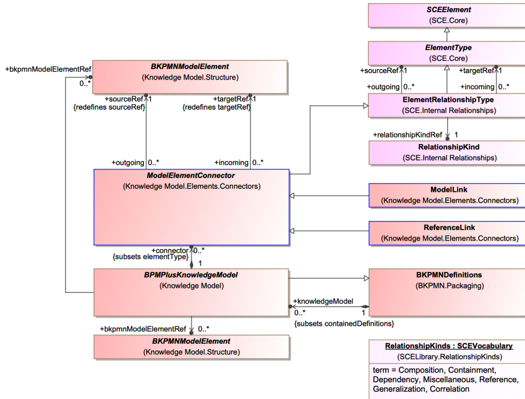
Figure 61: The Connectors Metamodel
