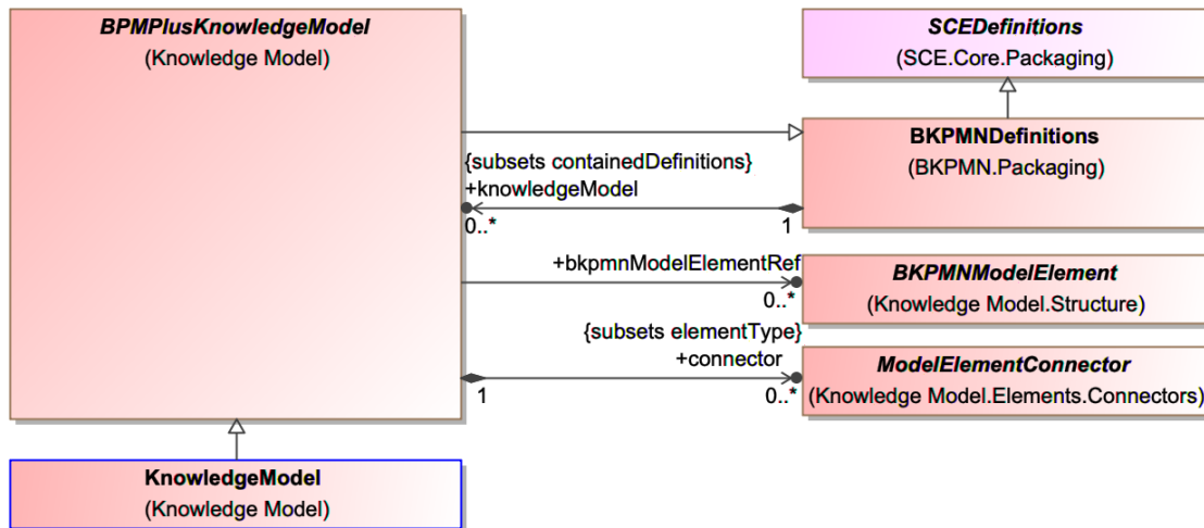
Figure 47: The BPMPlusKnowledgeModel Metamodel
