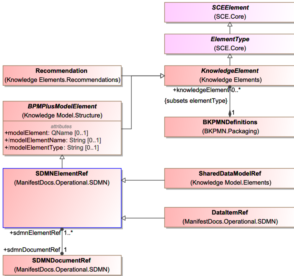
Figure 44: The SDMNElementRef Metamodel
