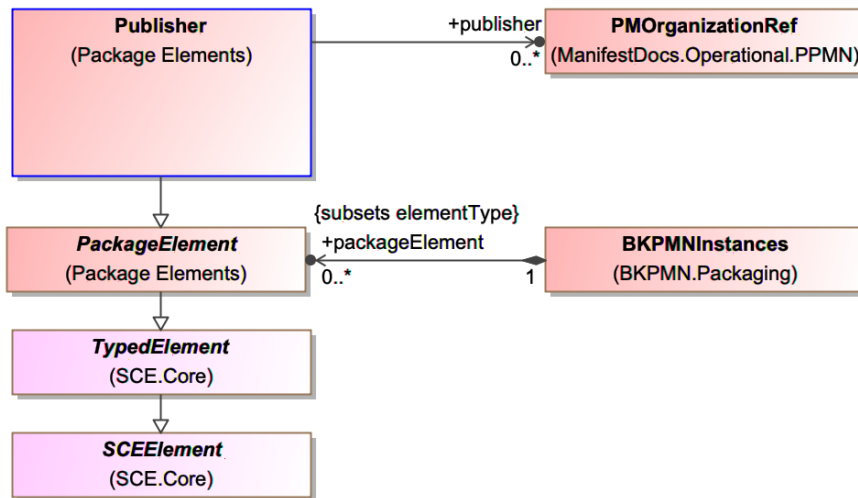
Figure 24: Publisher MM
