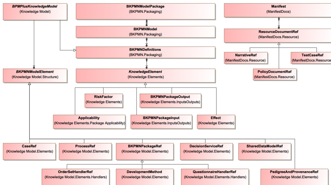
Figure 5: The BKPMN Package High Level Metamodel
