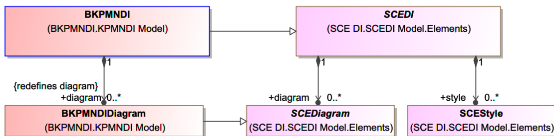
Figure 74: BKPMNDI
